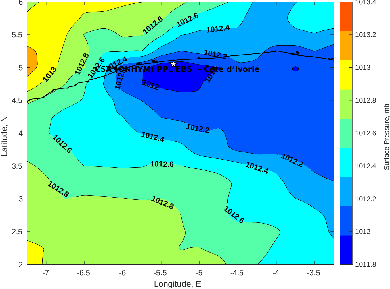
Surface Pressure (mb) for CSA (ONHYM) PPL EBS - Cote d'Ivoire at 23-Nov-2025 00:00:00
