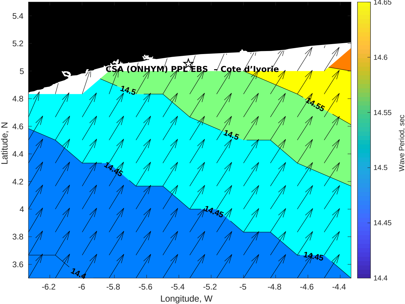
GFS Wave Period (sec) for CSA (ONHYM) PPL EBS - Cote d'Ivoire at 22-Nov-2025 09:00:00
