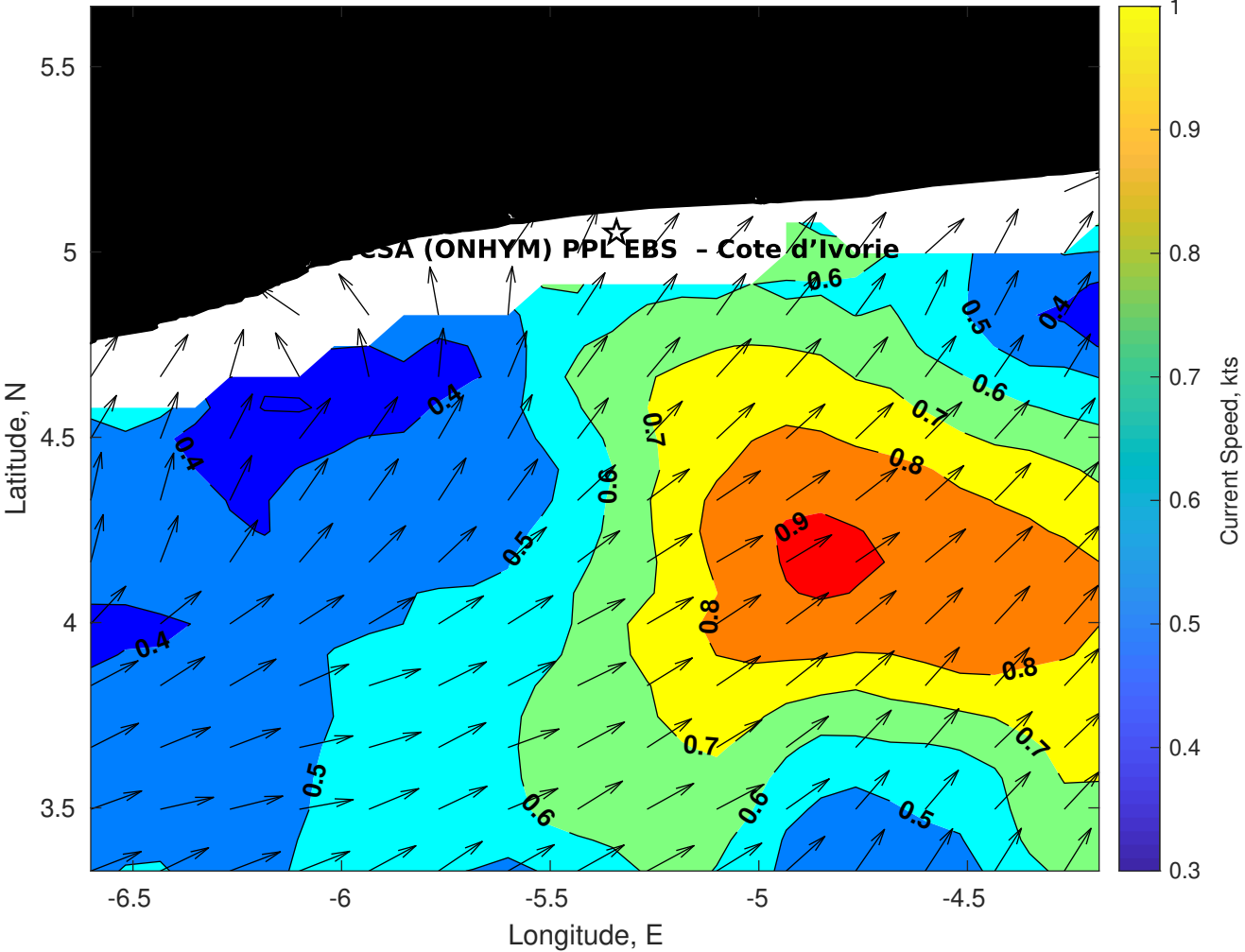
Surface Currents for CSA (ONHYM) PPL EBS - Cote d'Ivoire at 21-Nov-2025 00:00:00
