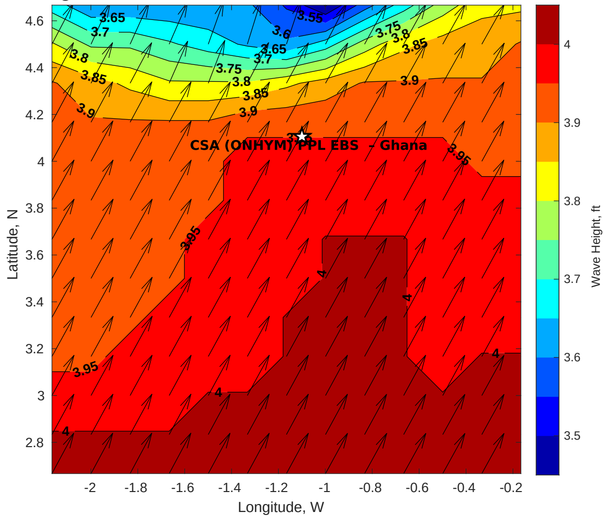
GFS Wave Height (ft) for CSA (ONHYM) PPL EBS - Ghana at 22-Nov-2025 09:00:00
