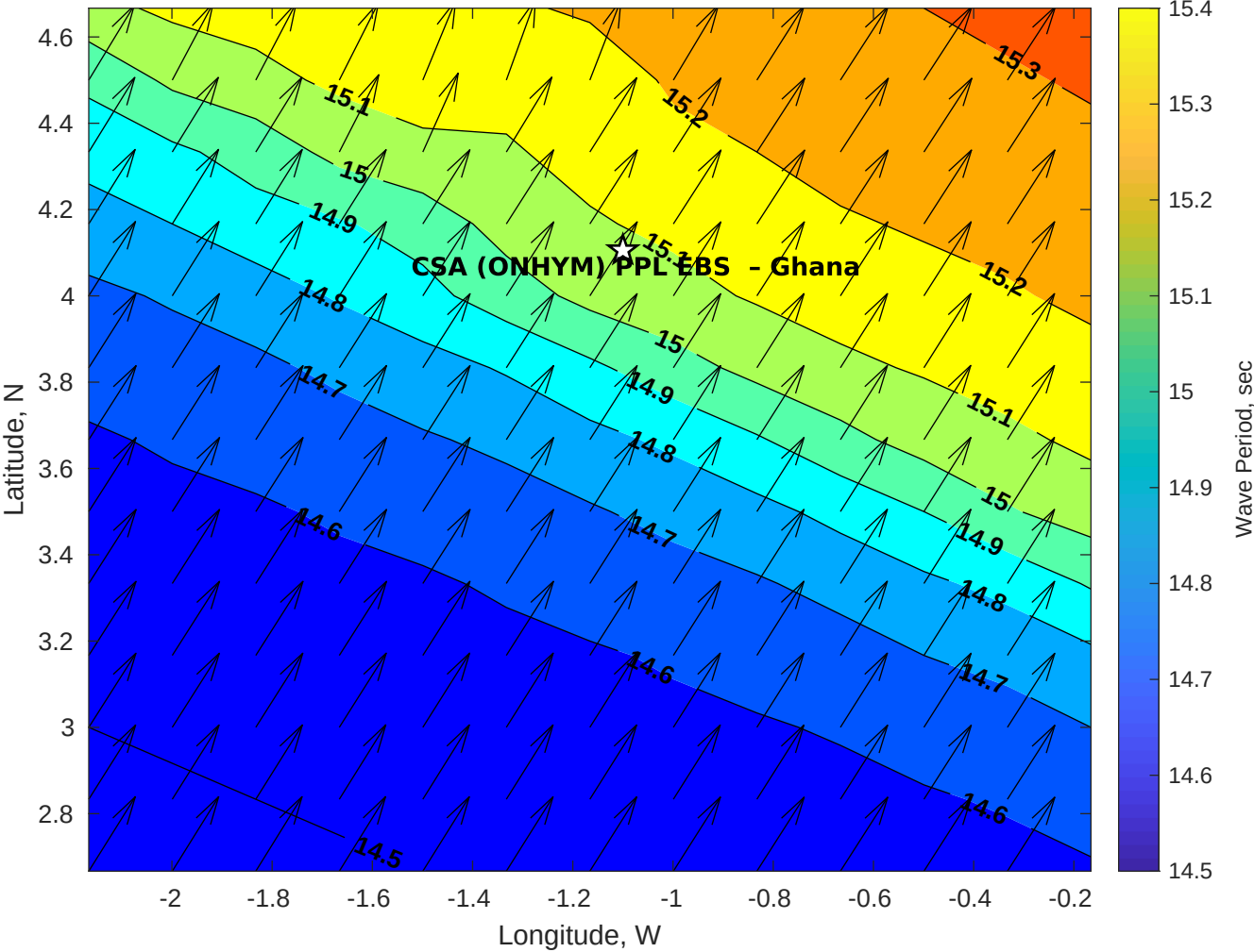
GFS Wave Period (sec) for CSA (ONHYM) PPL EBS - Ghana at 22-Nov-2025 09:00:00
