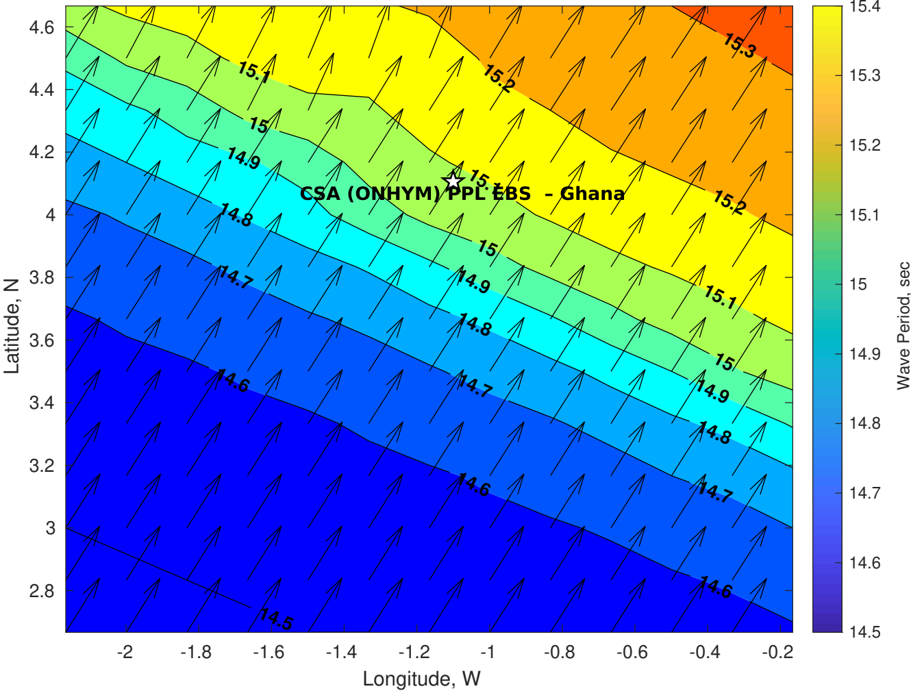
GFS Wave Period (sec) for CSA (ONHYM) PPL EBS - Ghana at 22-Nov-2025 09:00:00
