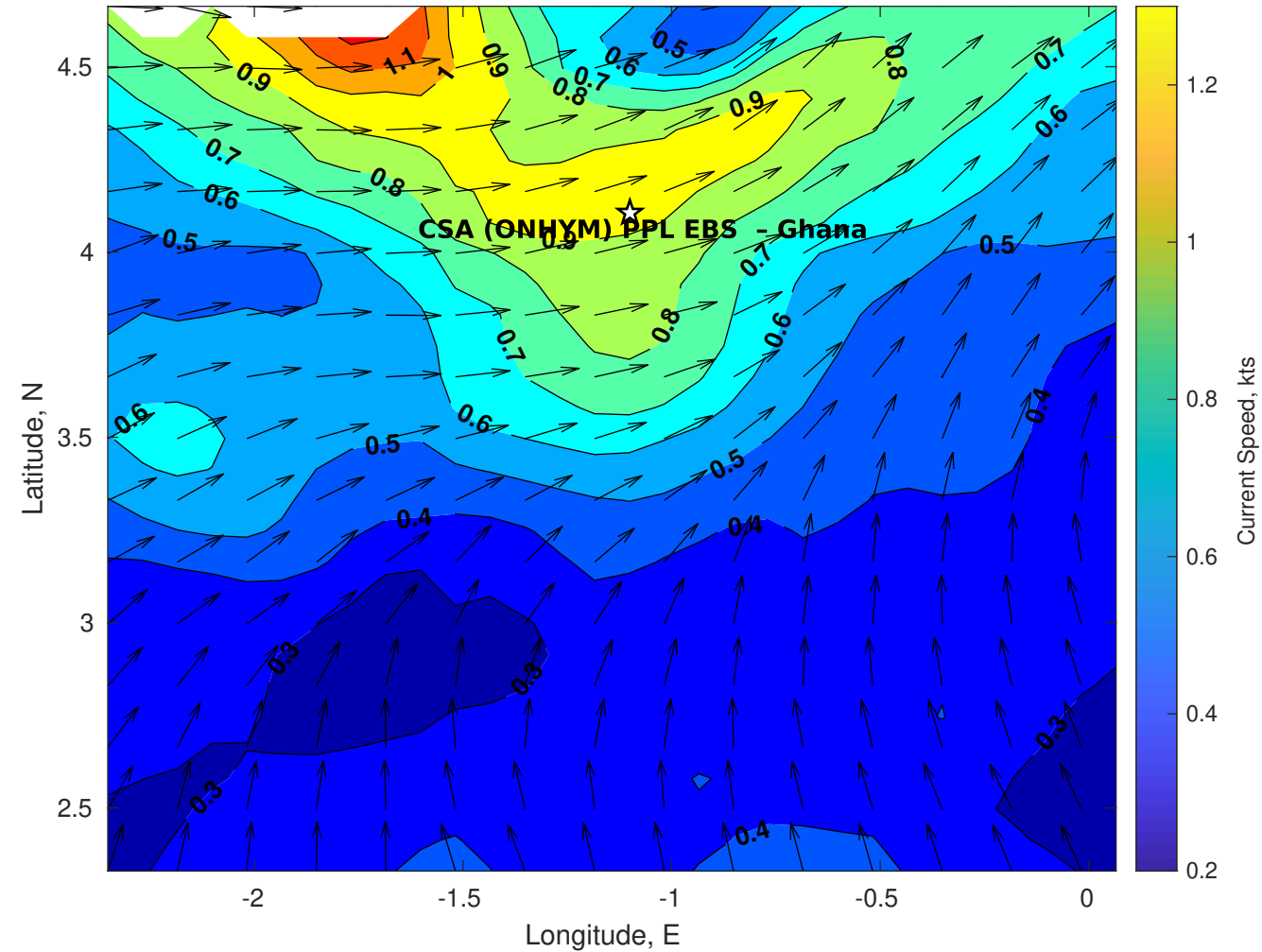
Surface Currents for CSA (ONHYM) PPL EBS - Ghana at 21-Nov-2025 00:00:00
