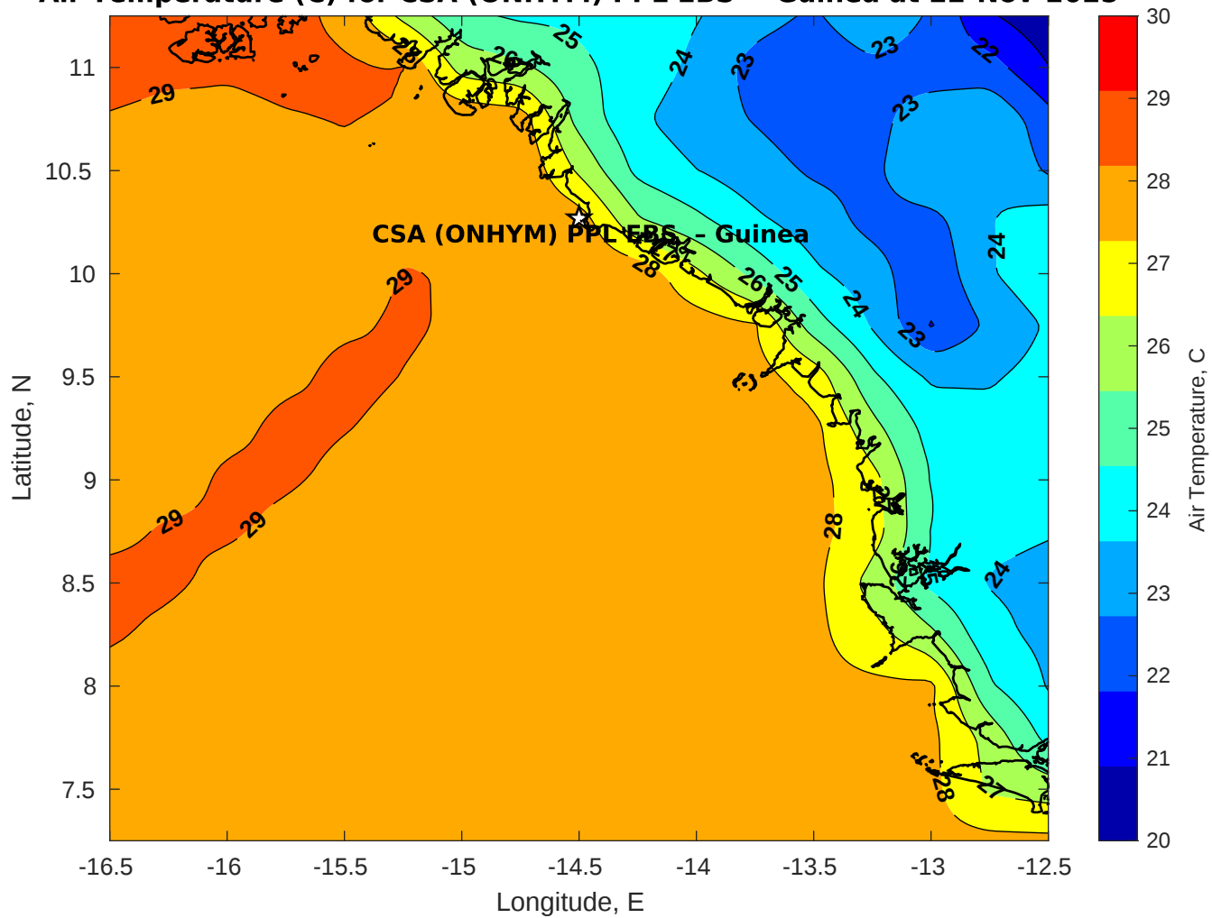
Air Temperature (C) for CSA (ONHYM) PPL EBS - Guinea at 22-Nov-2025
