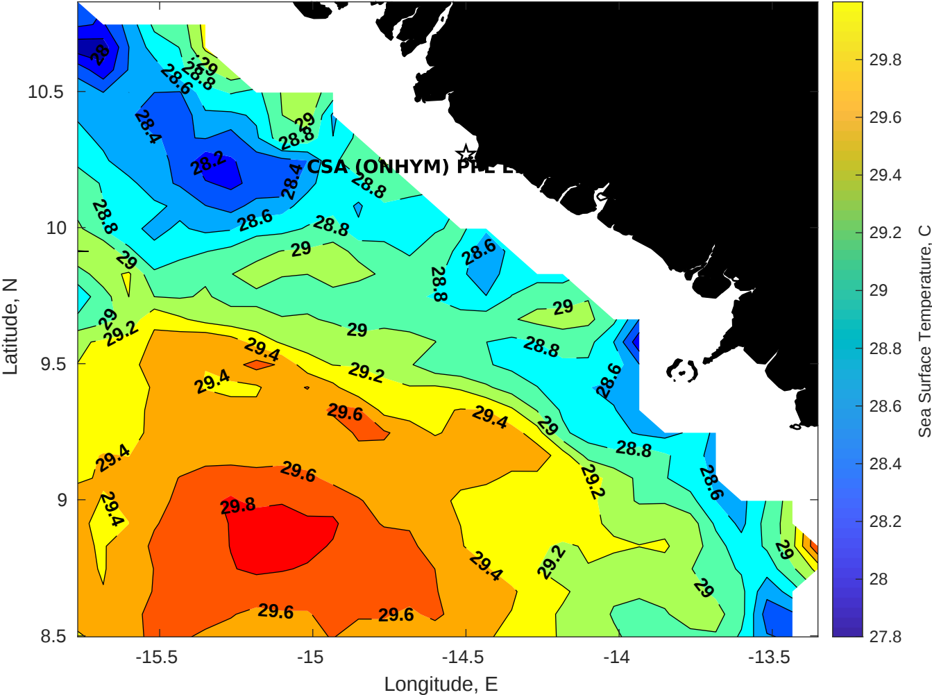
SST for CSA (ONHYM) PPL EBS - Guinea at 21-Nov-2025 00:00:00
