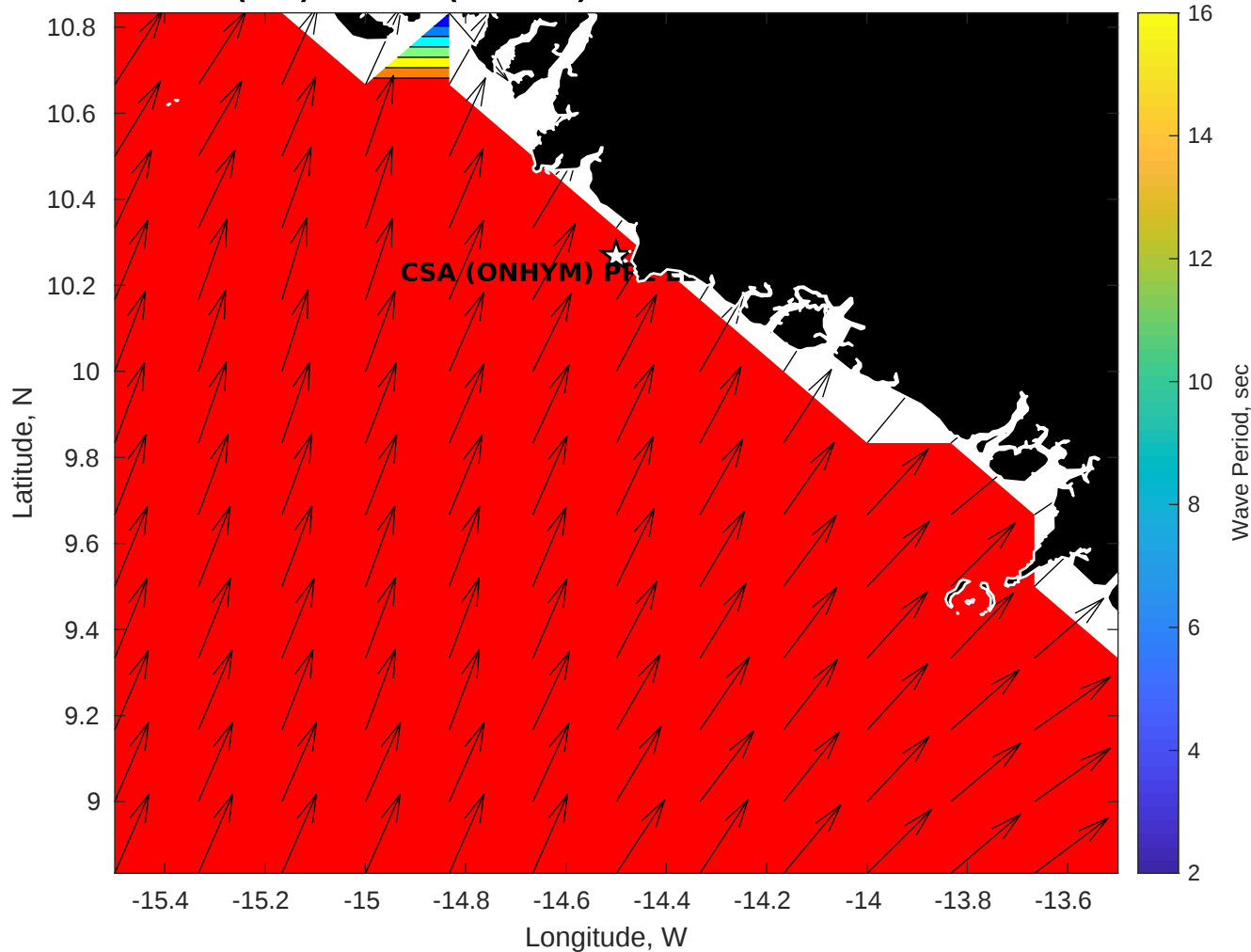
GFS Wave Period (sec) for CSA (ONHYM) PPL EBS - Guinea at 22-Nov-2025 09:00:00
