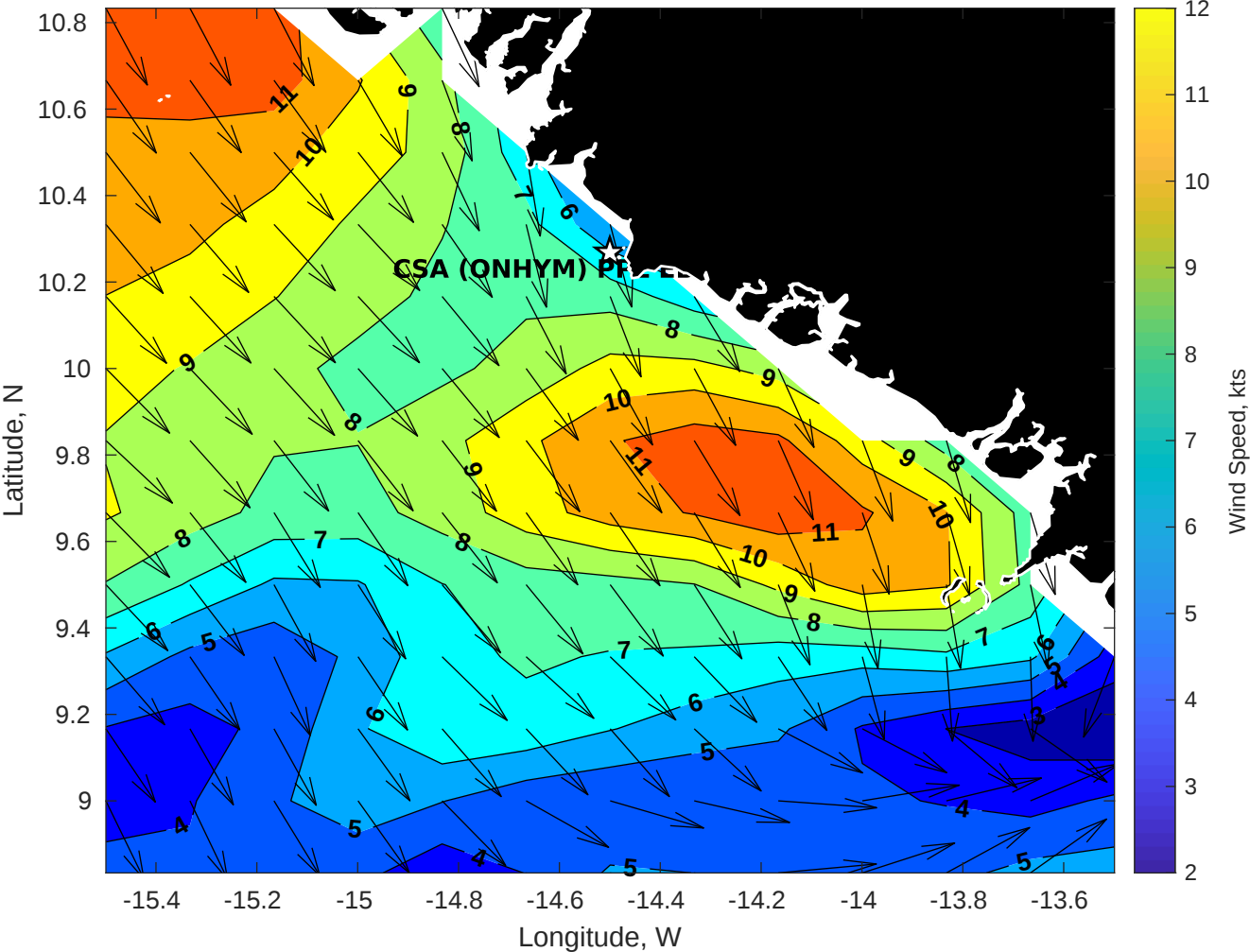
GFS Winds (kts) for CSA (ONHYM) PPL EBS - Guinea at 22-Nov-2025 09:00:00
