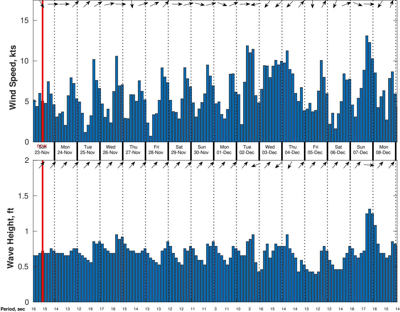
Wind & Wave Forecast for CSA (ONHYM) PPL EBS - Guinea from 22-Nov-2025 01:00:00 to 08-Dec-2025 01:00:00
