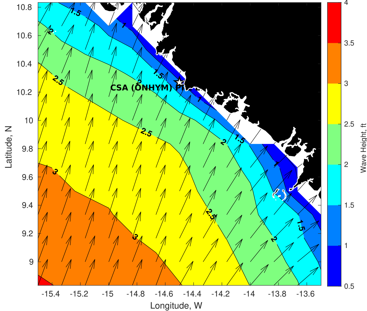
GFS Wave Height (ft) for CSA (ONHYM) PPL EBS - Guinea at 22-Nov-2025 09:00:00
