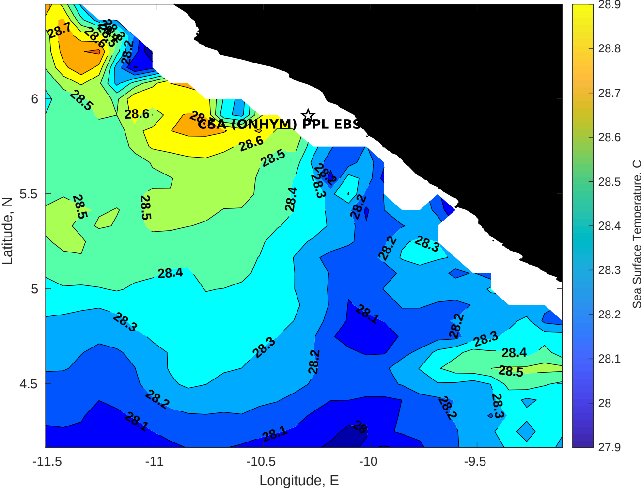
SST for CSA (ONHYM) PPL EBS - Liberia at 21-Nov-2025 00:00:00
