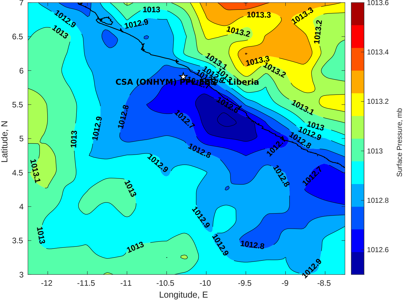
Surface Pressure (mb) for CSA (ONHYM) PPL EBS - Liberia at 22-Nov-2025 00:00:00
