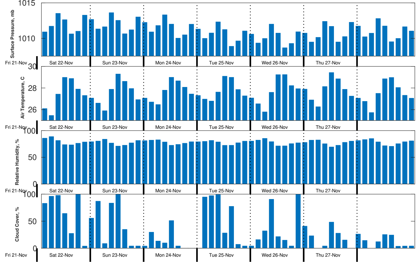
Met Forecast for CSA (ONHYM) PPL EBS - Liberia from 22-Nov-2025 00:00:00 to 29-Nov-2025 00:00:00
