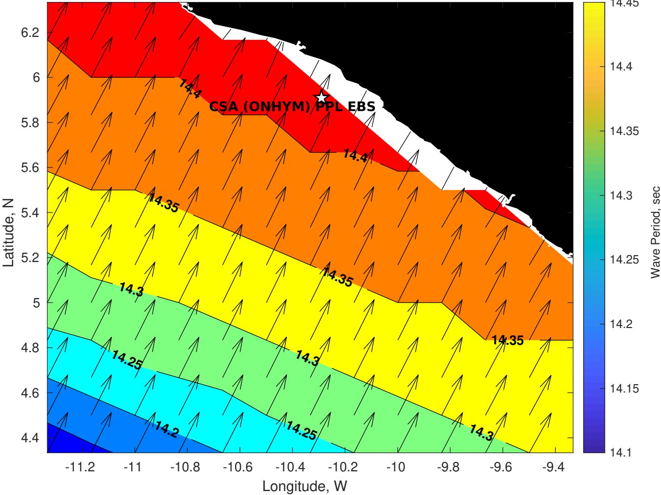
GFS Wave Period (sec) for CSA (ONHYM) PPL EBS - Liberia at 22-Nov-2025 09:00:00
