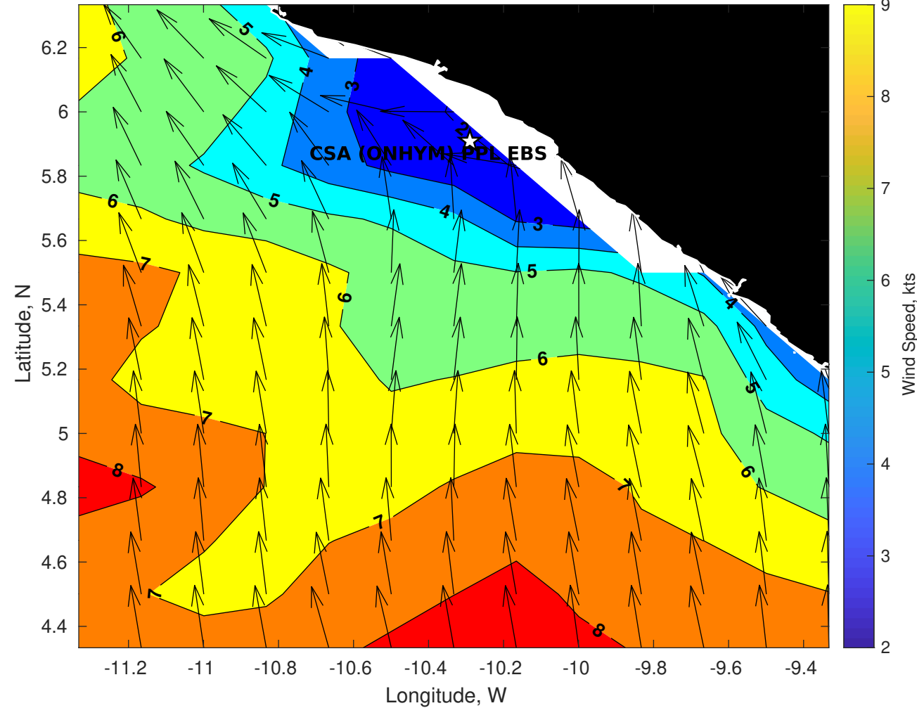
GFS Winds (kts) for CSA (ONHYM) PPL EBS - Liberia at 22-Nov-2025 09:00:00
