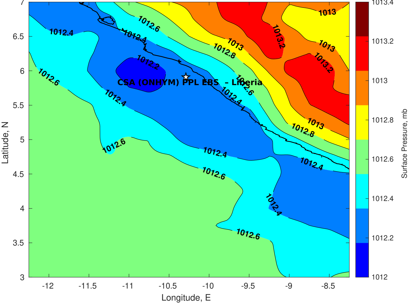
Surface Pressure (mb) for CSA (ONHYM) PPL EBS - Liberia at 24-Nov-2025 00:00:00
