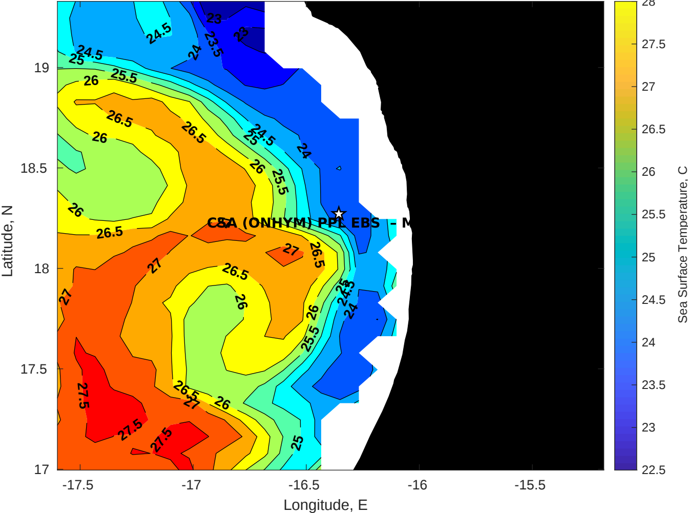
SST for CSA (ONHYM) PPL EBS - Mauritania at 21-Nov-2025 00:00:00
