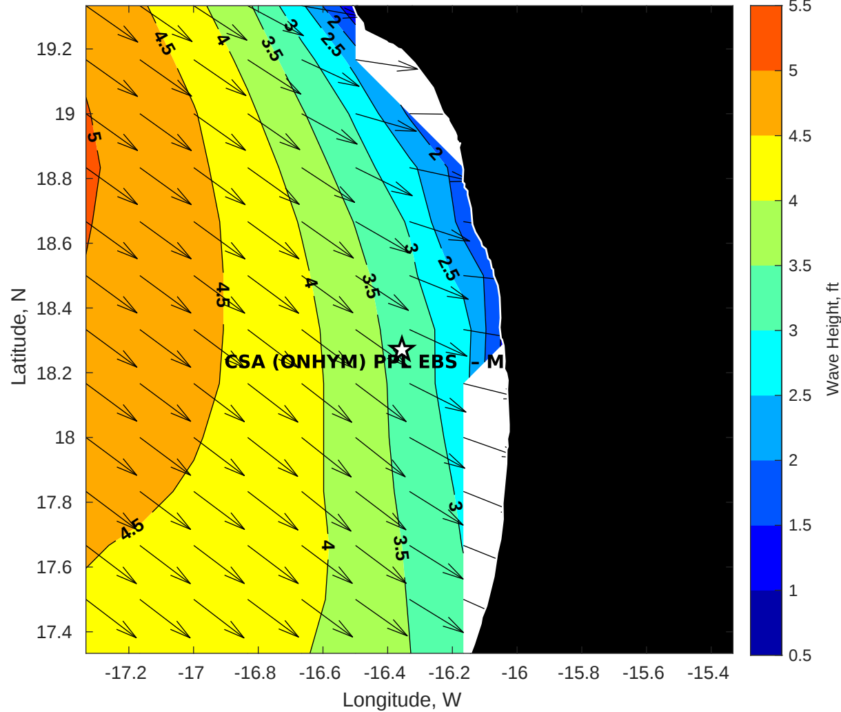
GFS Wave Height (ft) for CSA (ONHYM) PPL EBS - Mauritania at 22-Nov-2025 09:00:00
