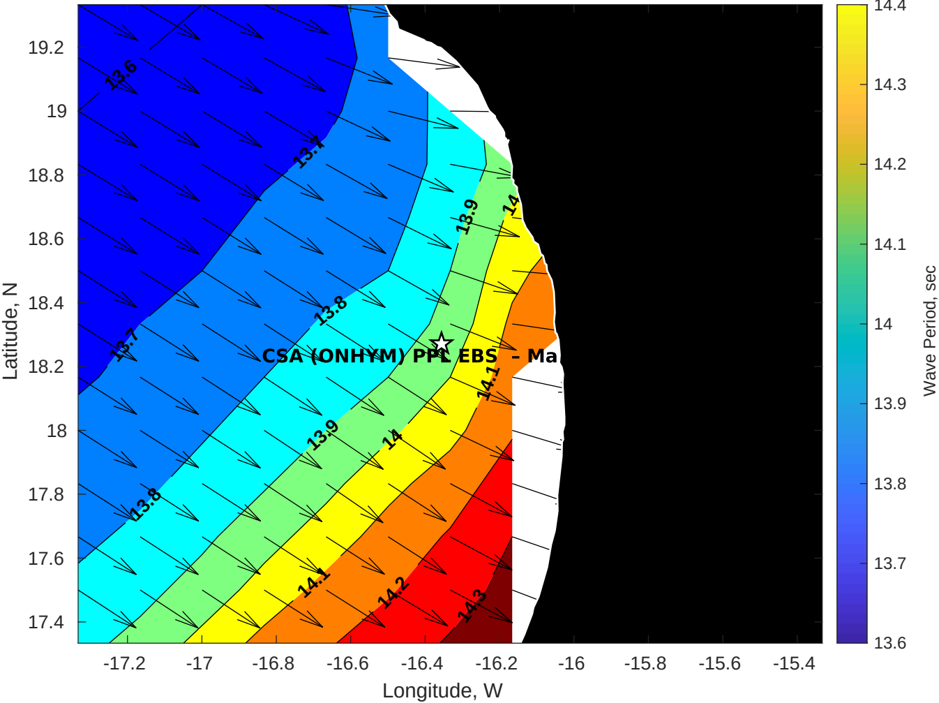
GFS Wave Period (sec) for CSA (ONHYM) PPL EBS - Mauritania at 22-Nov-2025 09:00:00
