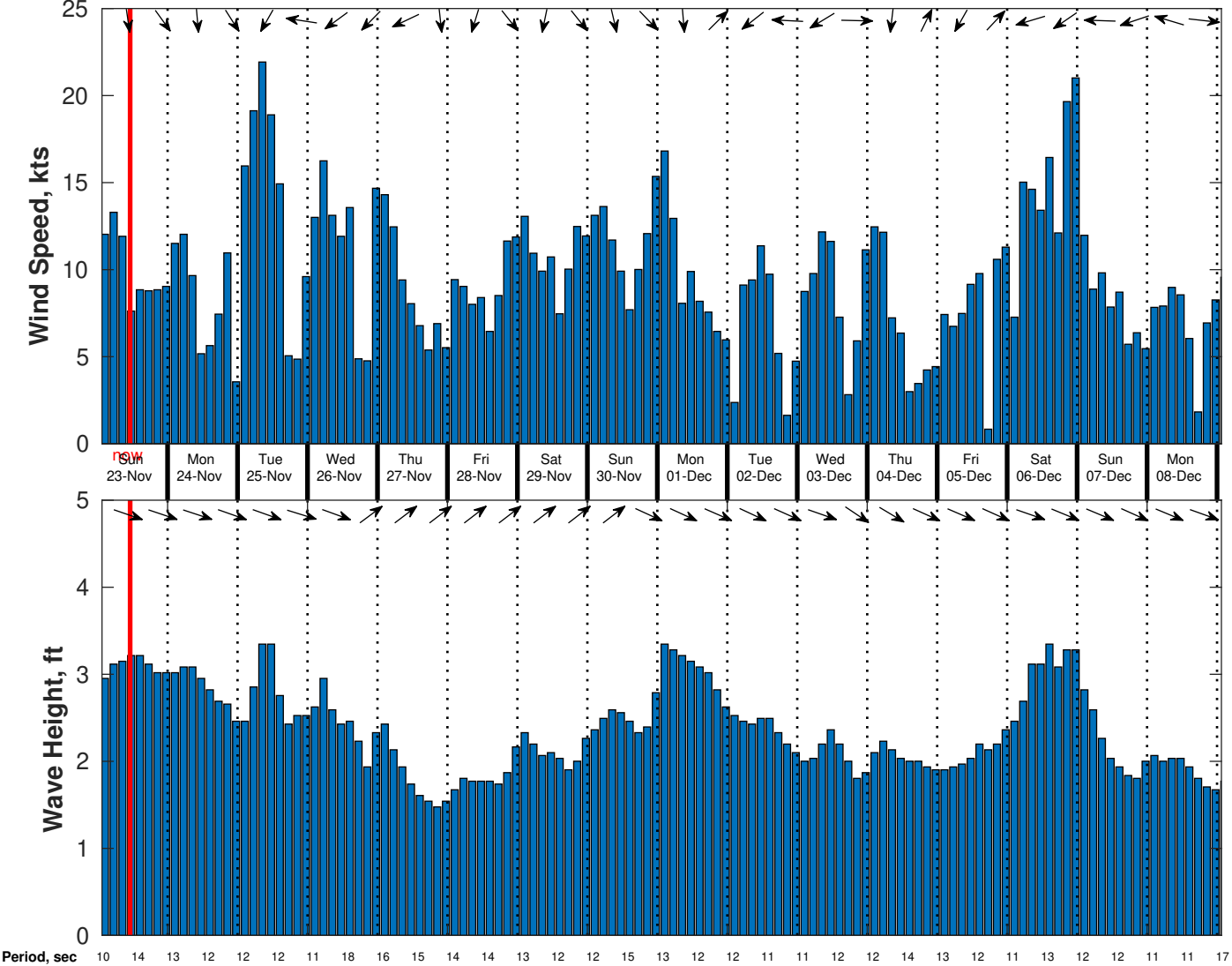
Wind & Wave Forecast for CSA (ONHYM) PPL EBS - Mauritania from 22-Nov-2025 01:00:00 to 08-Dec-2025 01:00:00
