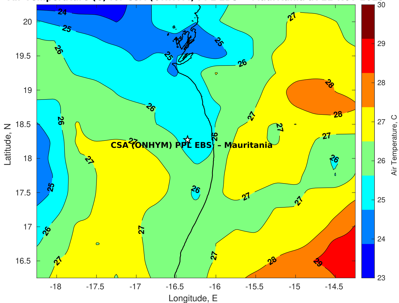
Air Temperature (C) for CSA (ONHYM) PPL EBS - Mauritania at 22-Nov-2025
