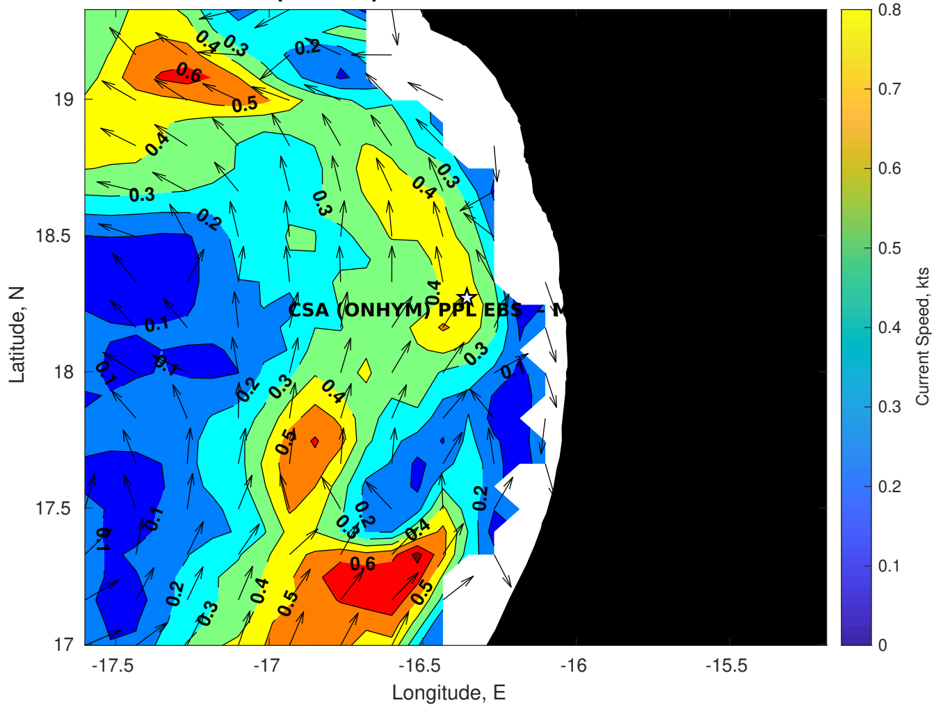
Surface Currents for CSA (ONHYM) PPL EBS - Mauritania at 21-Nov-2025 00:00:00
