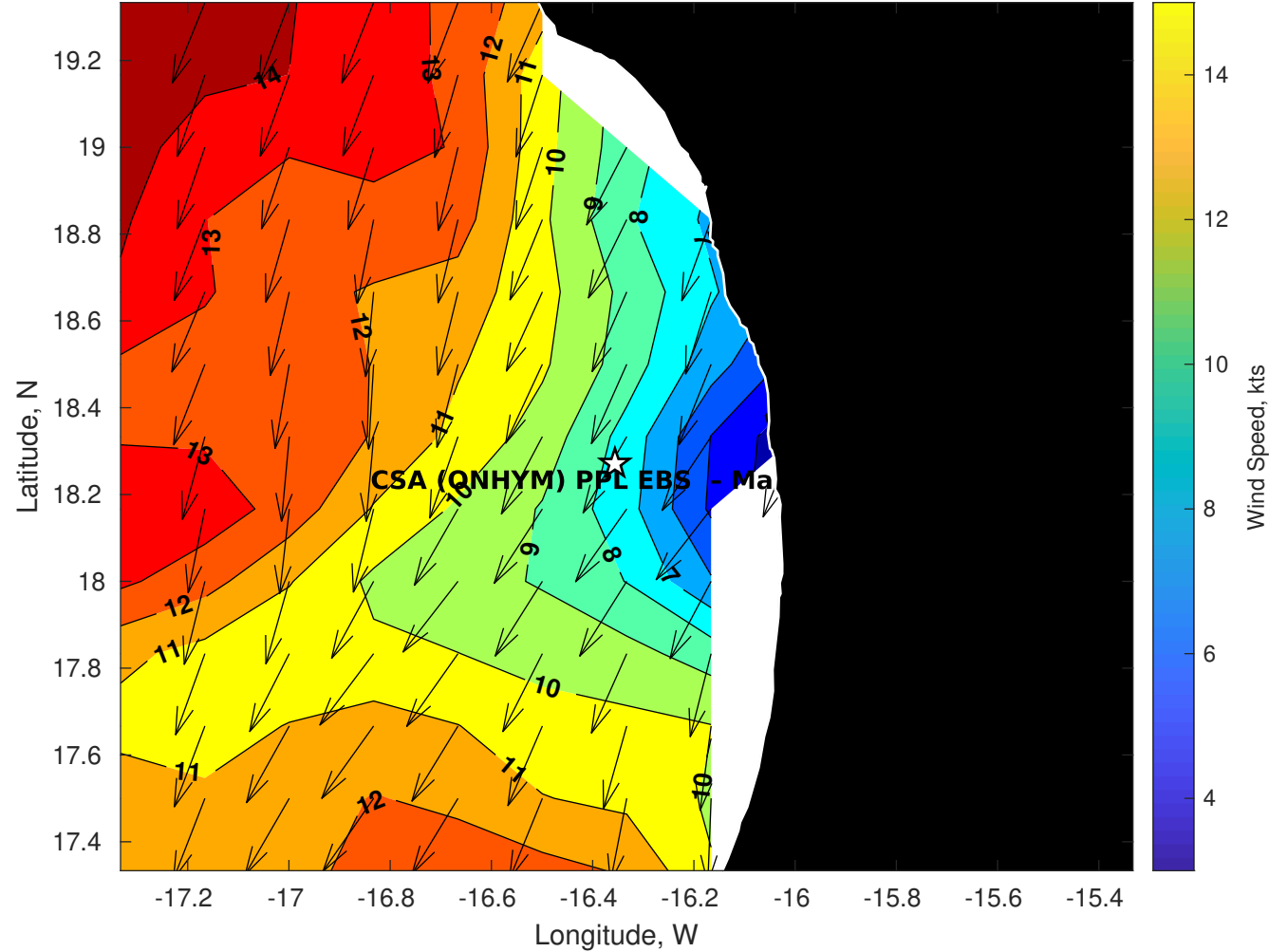
GFS Winds (kts) for CSA (ONHYM) PPL EBS - Mauritania at 22-Nov-2025 09:00:00
