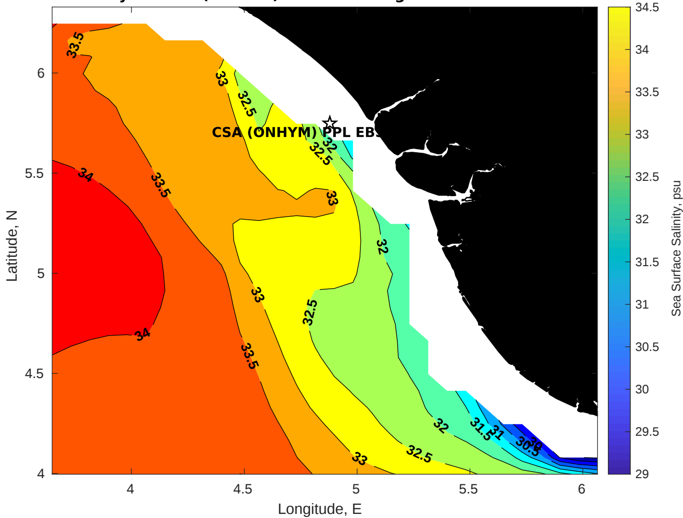
Surface Salinity for CSA (ONHYM) PPL EBS - Nigeria at 21-Nov-2025 00:00:00
