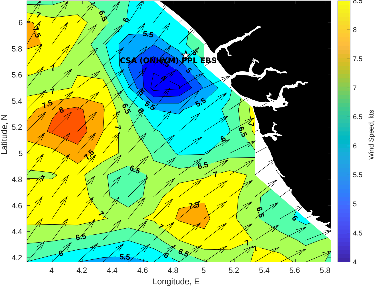
GFS Winds (kts) for CSA (ONHYM) PPL EBS - Nigeria at 22-Nov-2025 09:00:00
