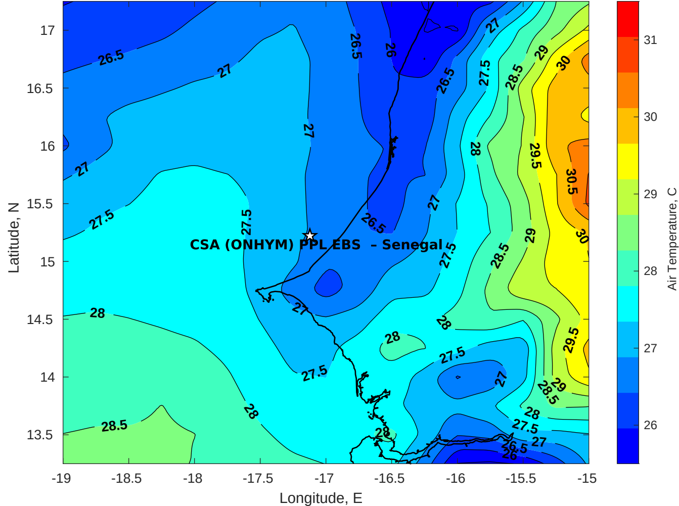
Air Temperature (C) for CSA (ONHYM) PPL EBS - Senegal at 22-Nov-2025
