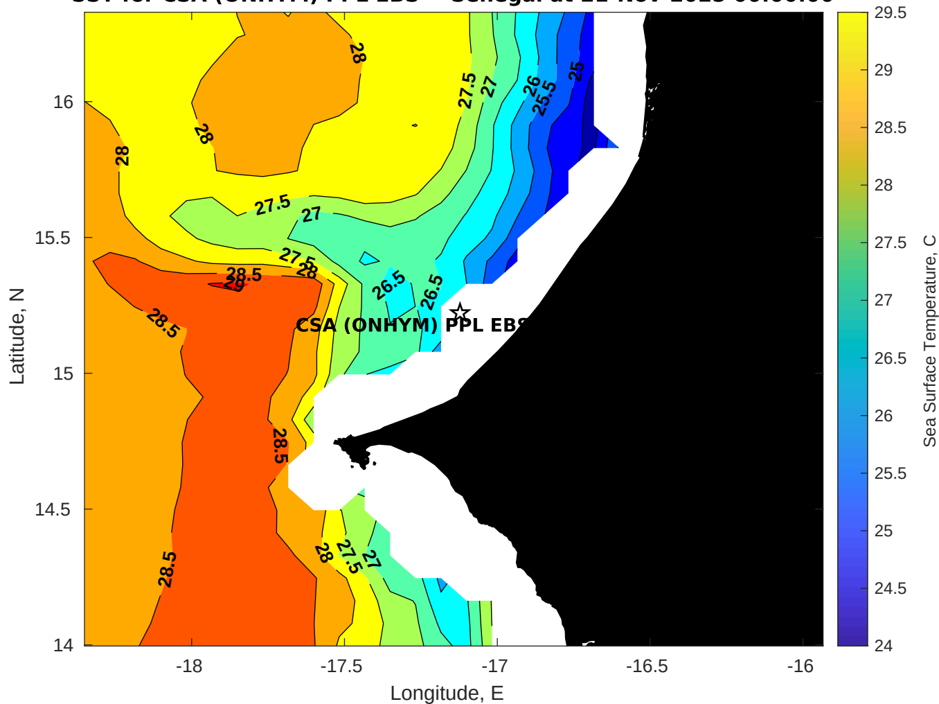
SST for CSA (ONHYM) PPL EBS - Senegal at 21-Nov-2025 00:00:00
