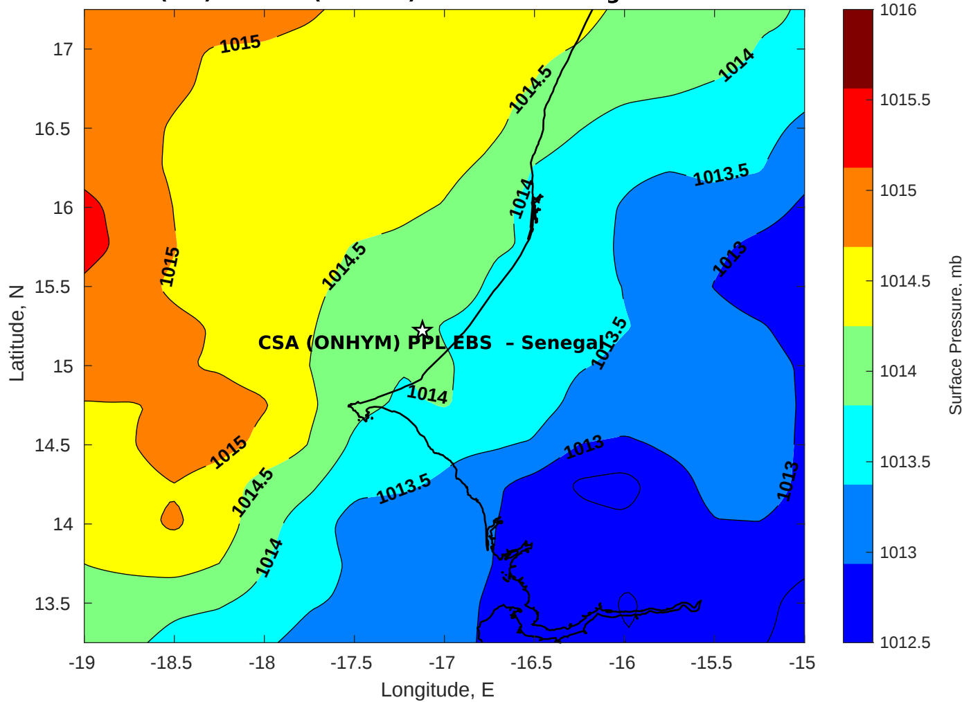
Surface Pressure (mb) for CSA (ONHYM) PPL EBS - Senegal at 23-Nov-2025 00:00:00
