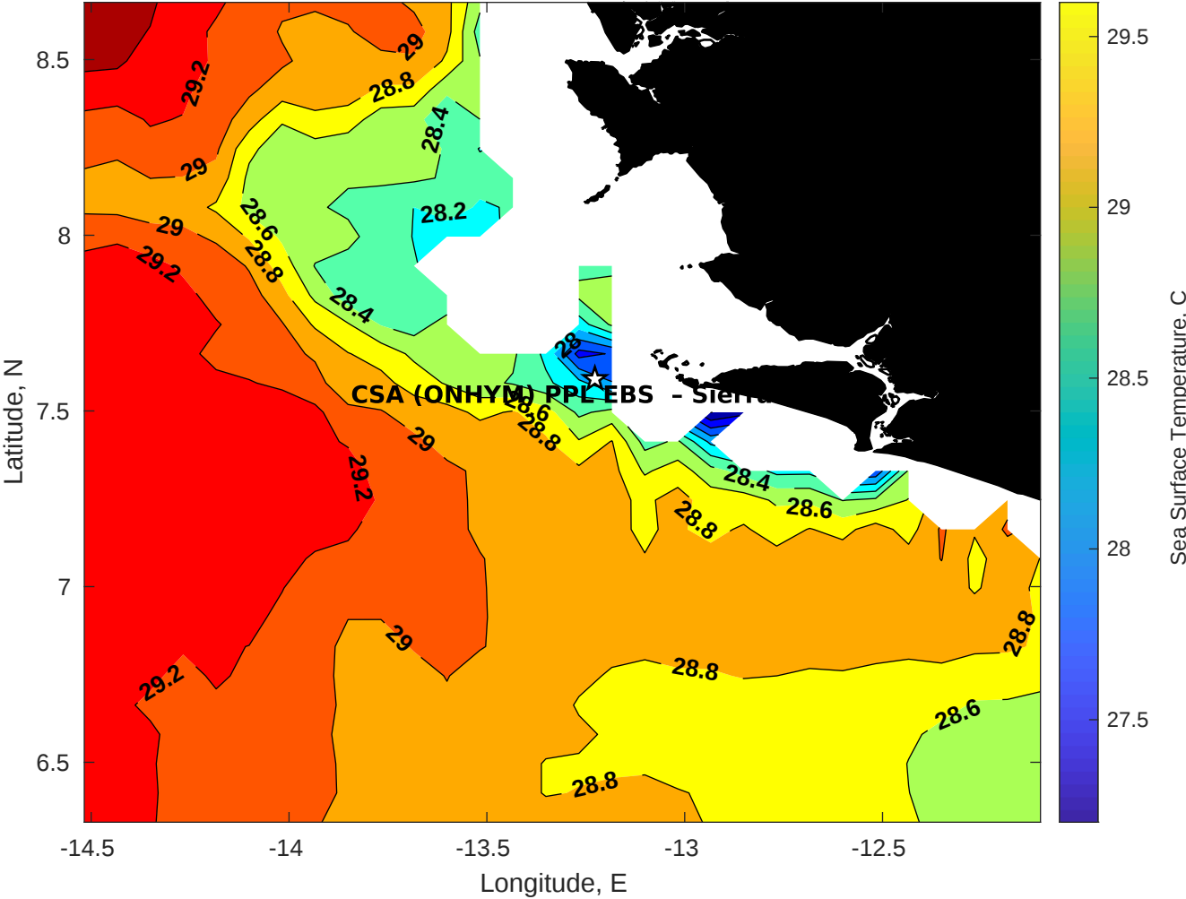
SST for CSA (ONHYM) PPL EBS - Sierra Leone at 21-Nov-2025 00:00:00
