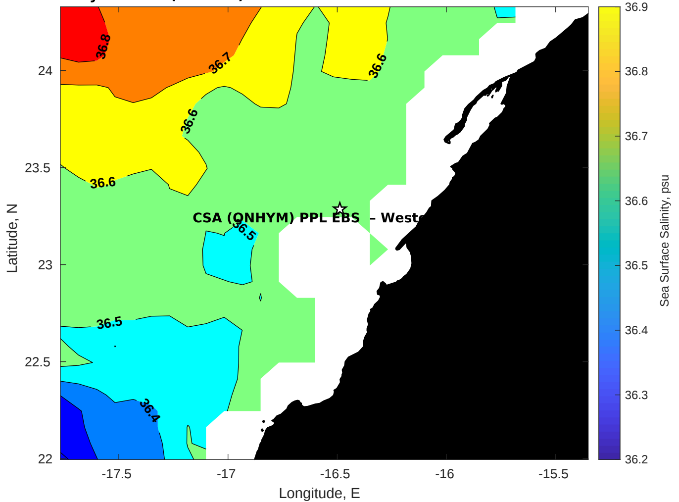
Surface Salinity for CSA (ONHYM) PPL EBS - Western Sahara at 21-Nov-2025 00:00:00
