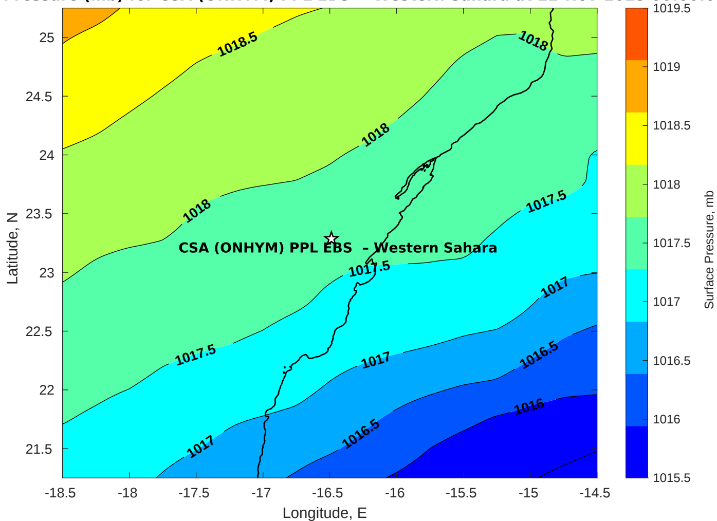
Surface Pressure (mb) for CSA (ONHYM) PPL EBS - Western Sahara at 22-Nov-2025 00:00:00
