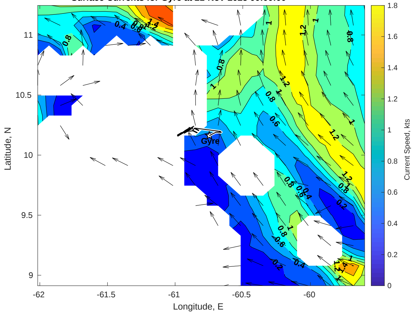
Surface Currents for Gyre at 21-Nov-2025 00:00:00
