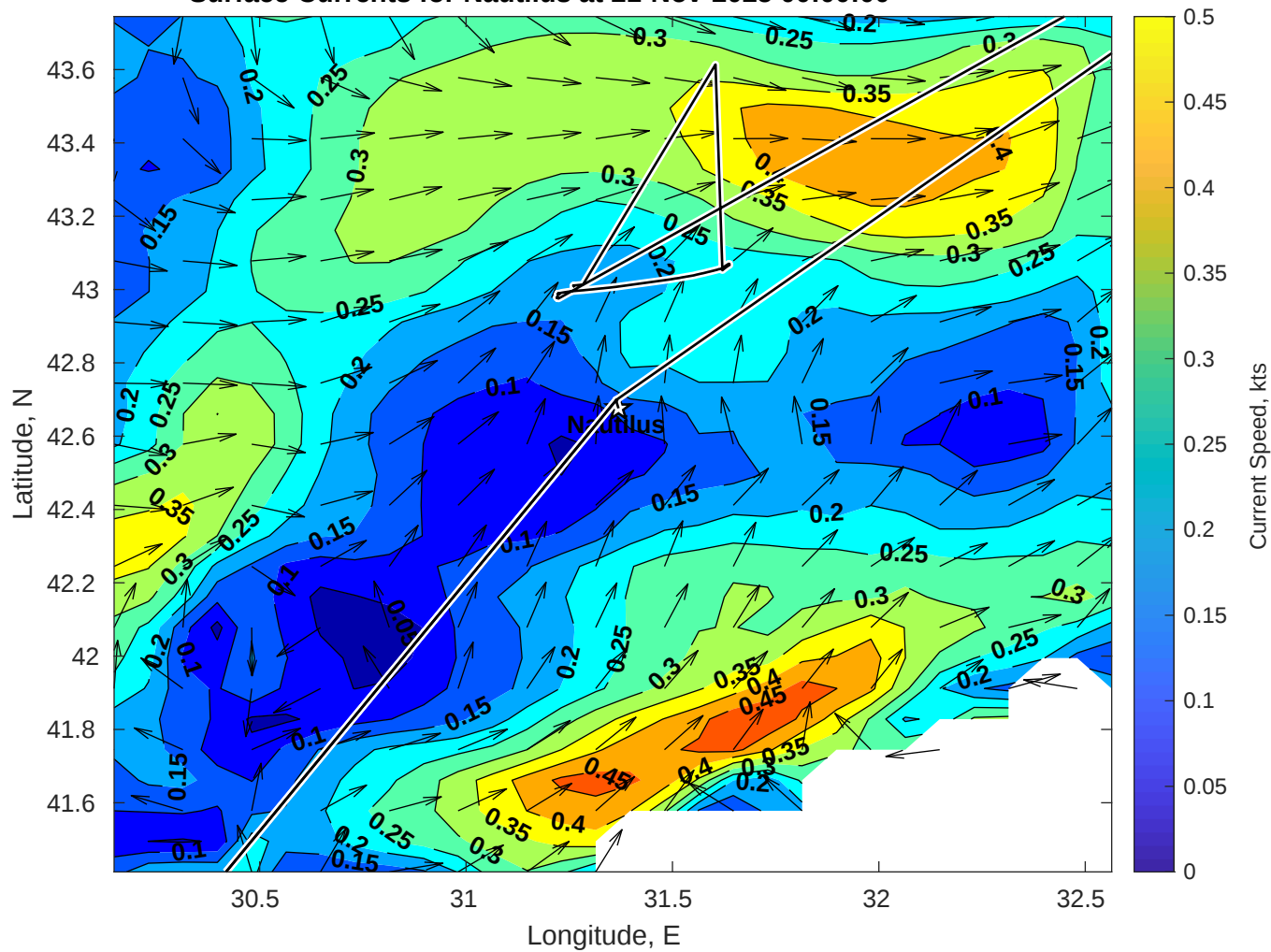
Surface Currents for Nautilus at 21-Nov-2025 00:00:00
