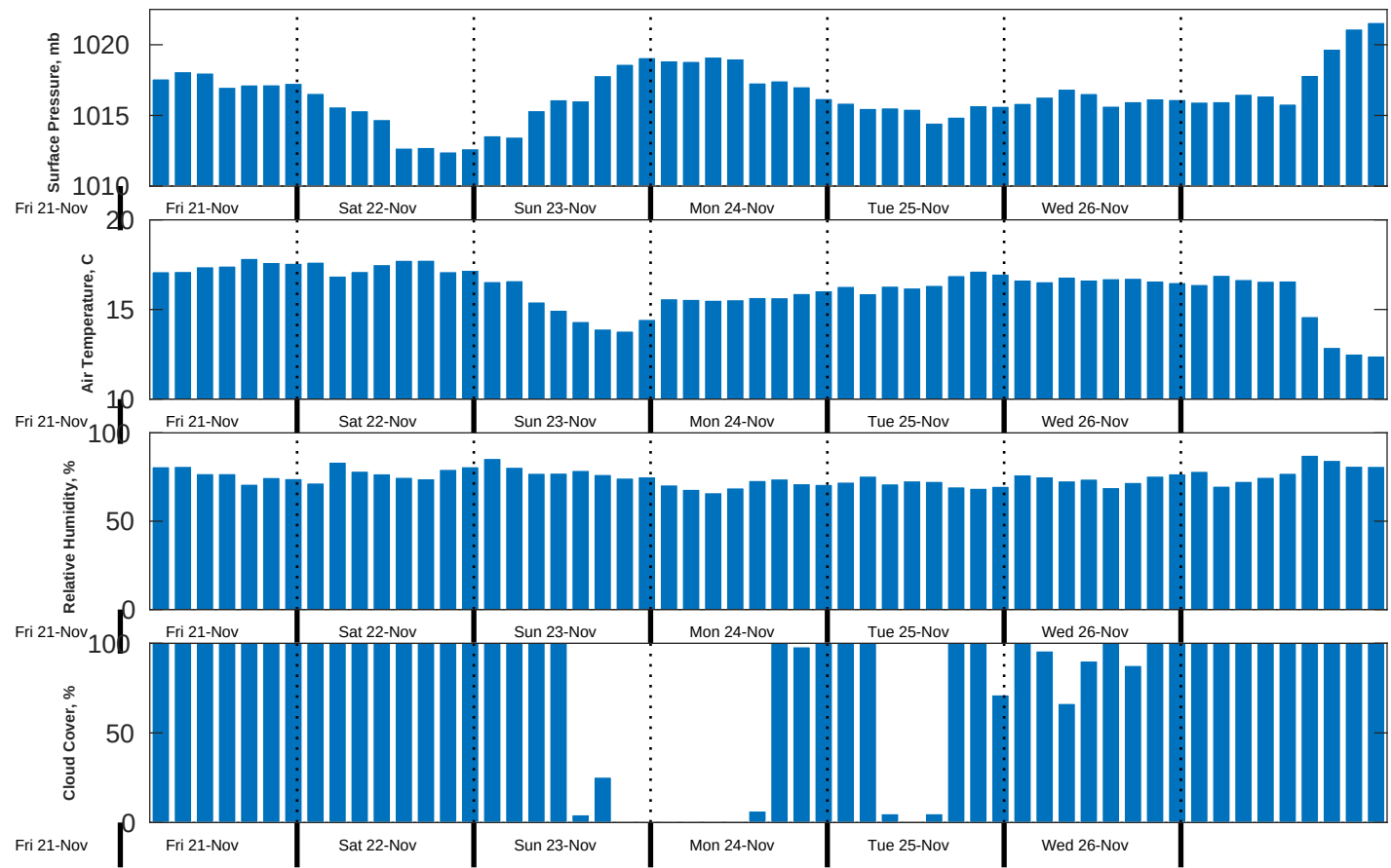
Met Forecast for Nautilus from 22-Nov-2025 00:00:00 to 29-Nov-2025 00:00:00
