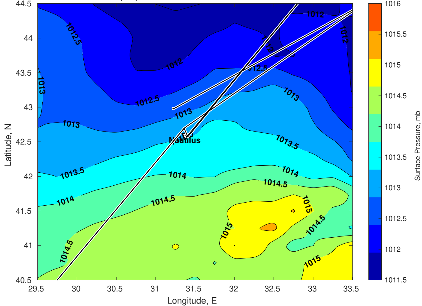
Surface Pressure (mb) for Nautilus at 24-Nov-2025 00:00:00
