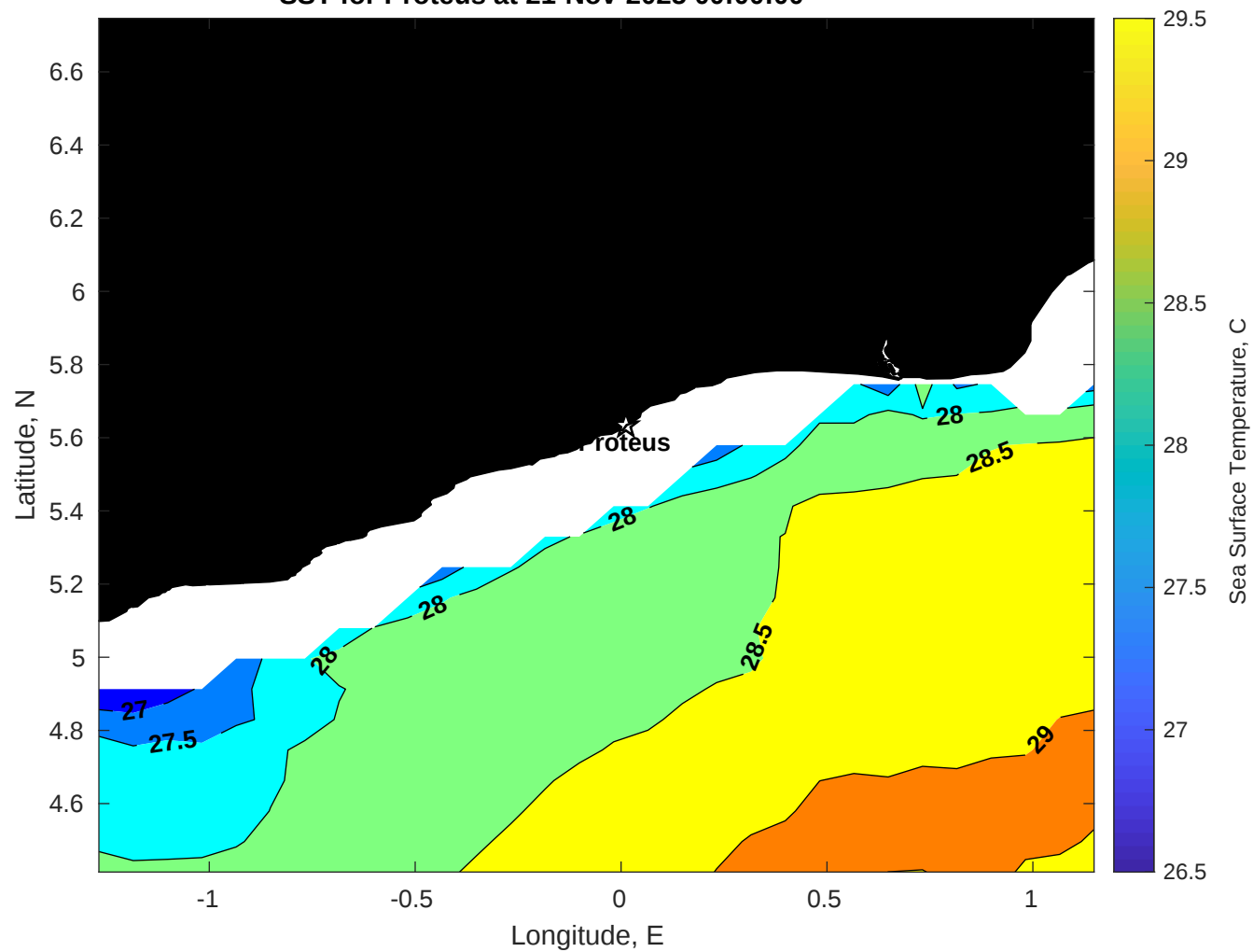
SST for Proteus at 21-Nov-2025 00:00:00
