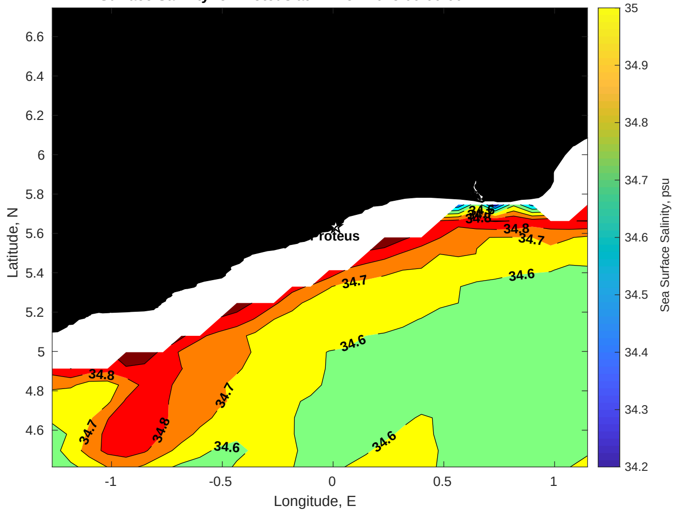
Surface Salinity for Proteus at 21-Nov-2025 00:00:00
