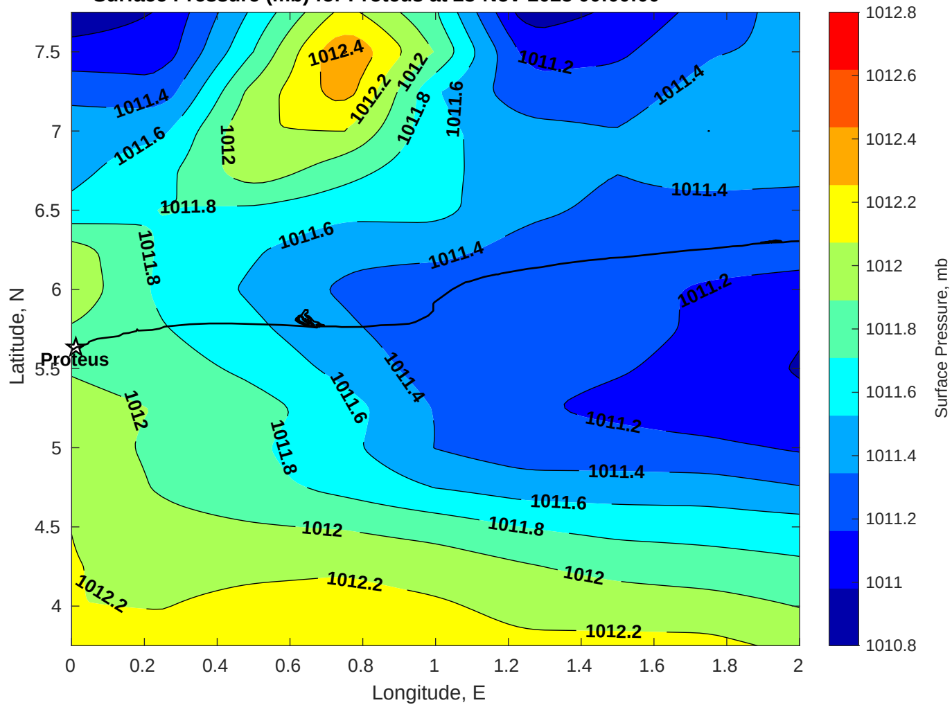
Surface Pressure (mb) for Proteus at 23-Nov-2025 00:00:00
