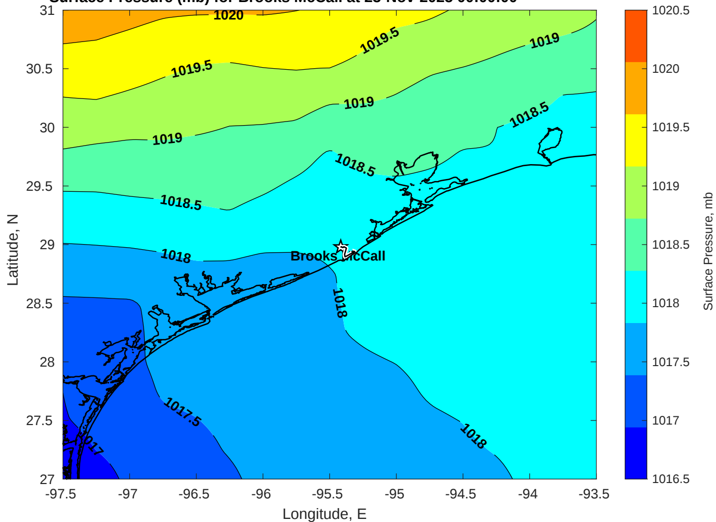
Surface Pressure (mb) for Brooks McCall at 23-Nov-2025 00:00:00
