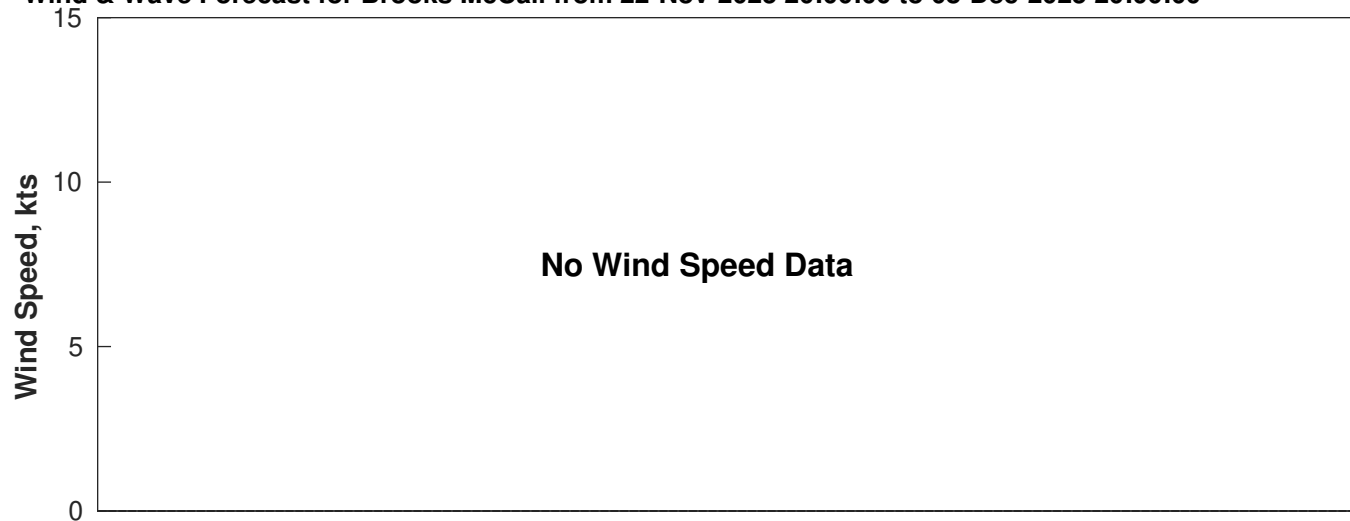
Wind & Wave Forecast for Brooks McCall from 22-Nov-2025 20:00:00 to 08-Dec-2025 20:00:00
