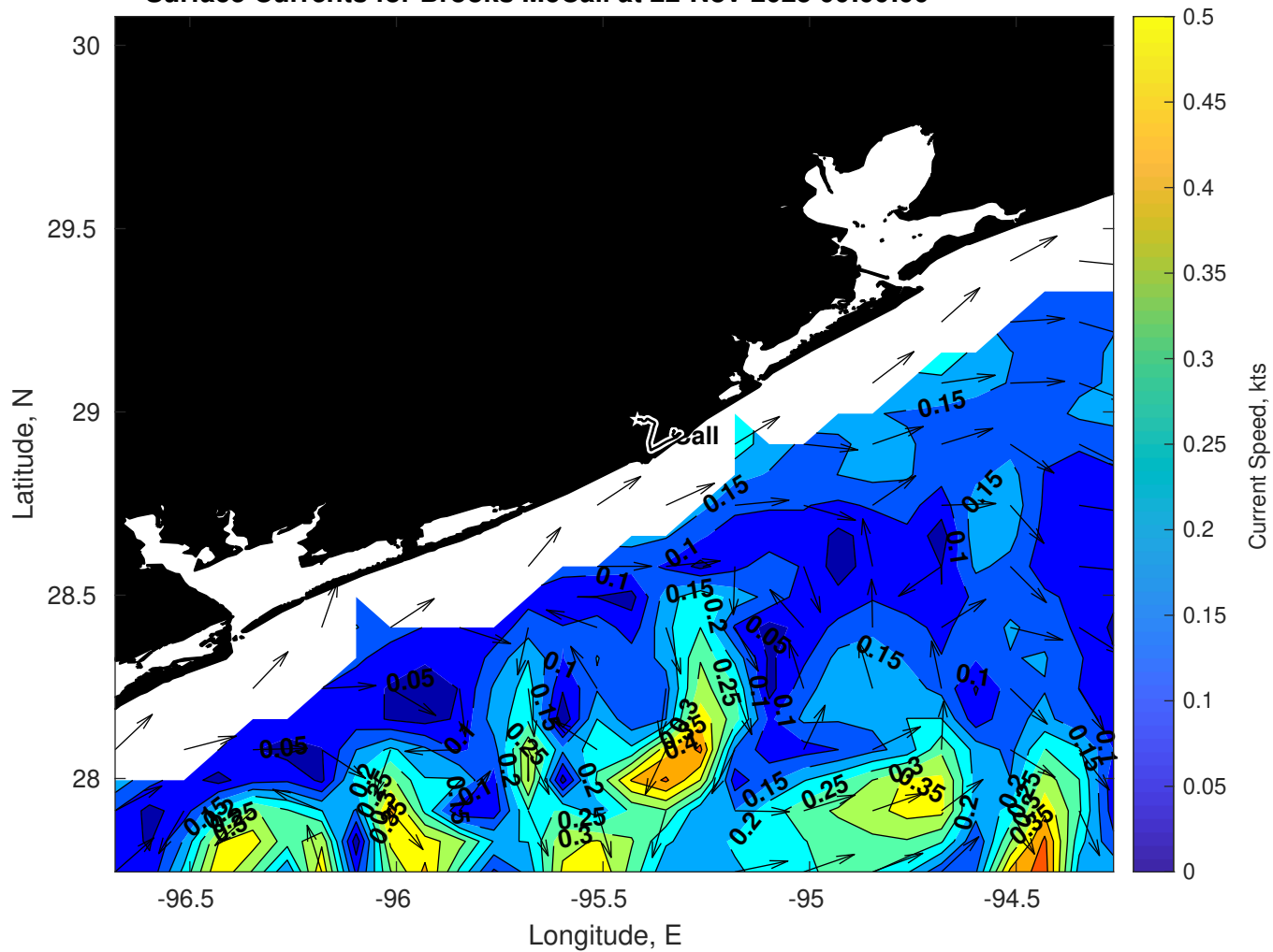
Surface Currents for Brooks McCall at 22-Nov-2025 00:00:00
