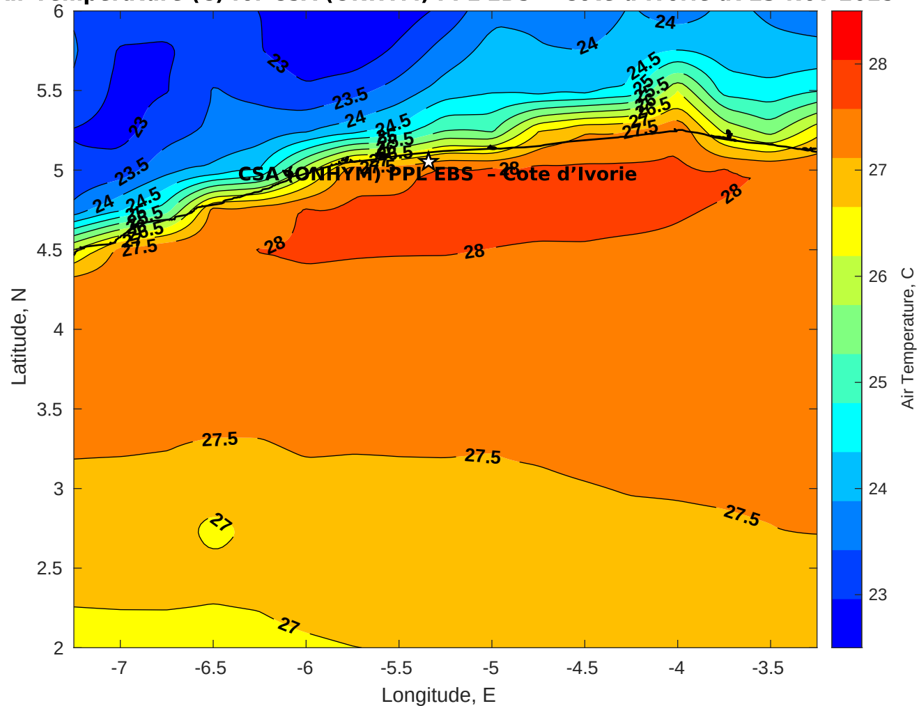
Air Temperature (C) for CSA (ONHYM) PPL EBS - Cote d'Ivoire at 23-Nov-2025
