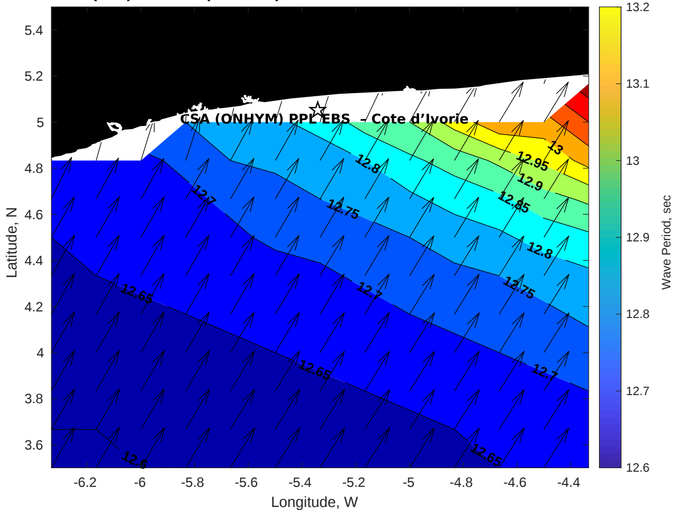
GFS Wave Period (sec) for CSA (ONHYM) PPL EBS - Cote d'Ivoire at 23-Nov-2025 09:00:00
