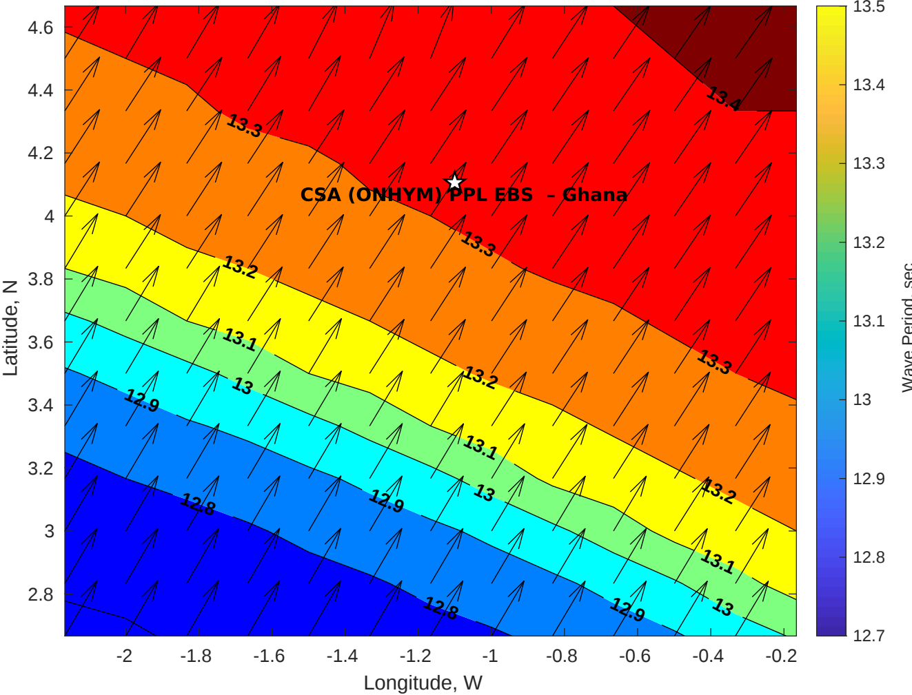
GFS Wave Period (sec) for CSA (ONHYM) PPL EBS - Ghana at 23-Nov-2025 09:00:00
