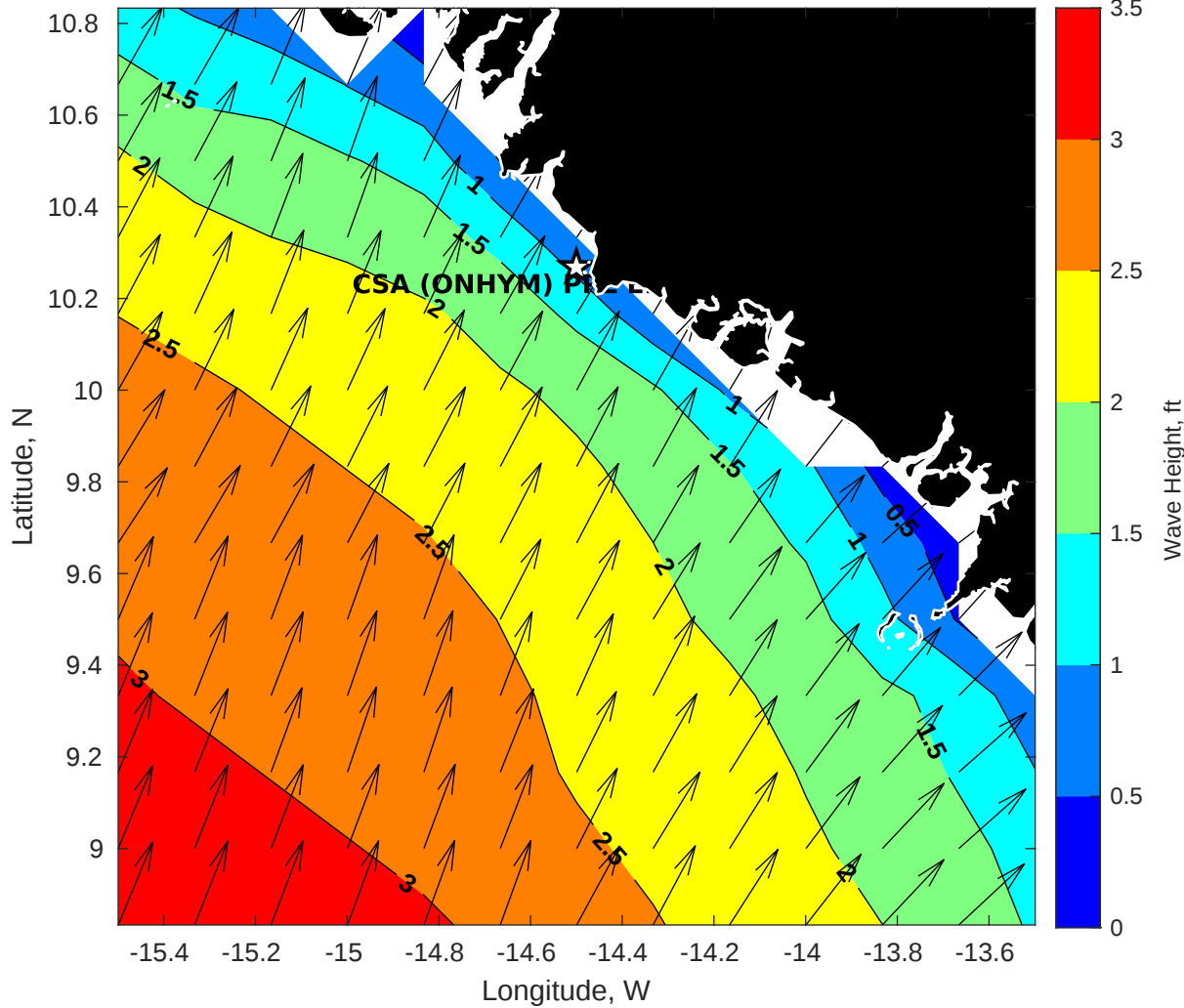
GFS Wave Height (ft) for CSA (ONHYM) PPL EBS - Guinea at 23-Nov-2025 09:00:00
