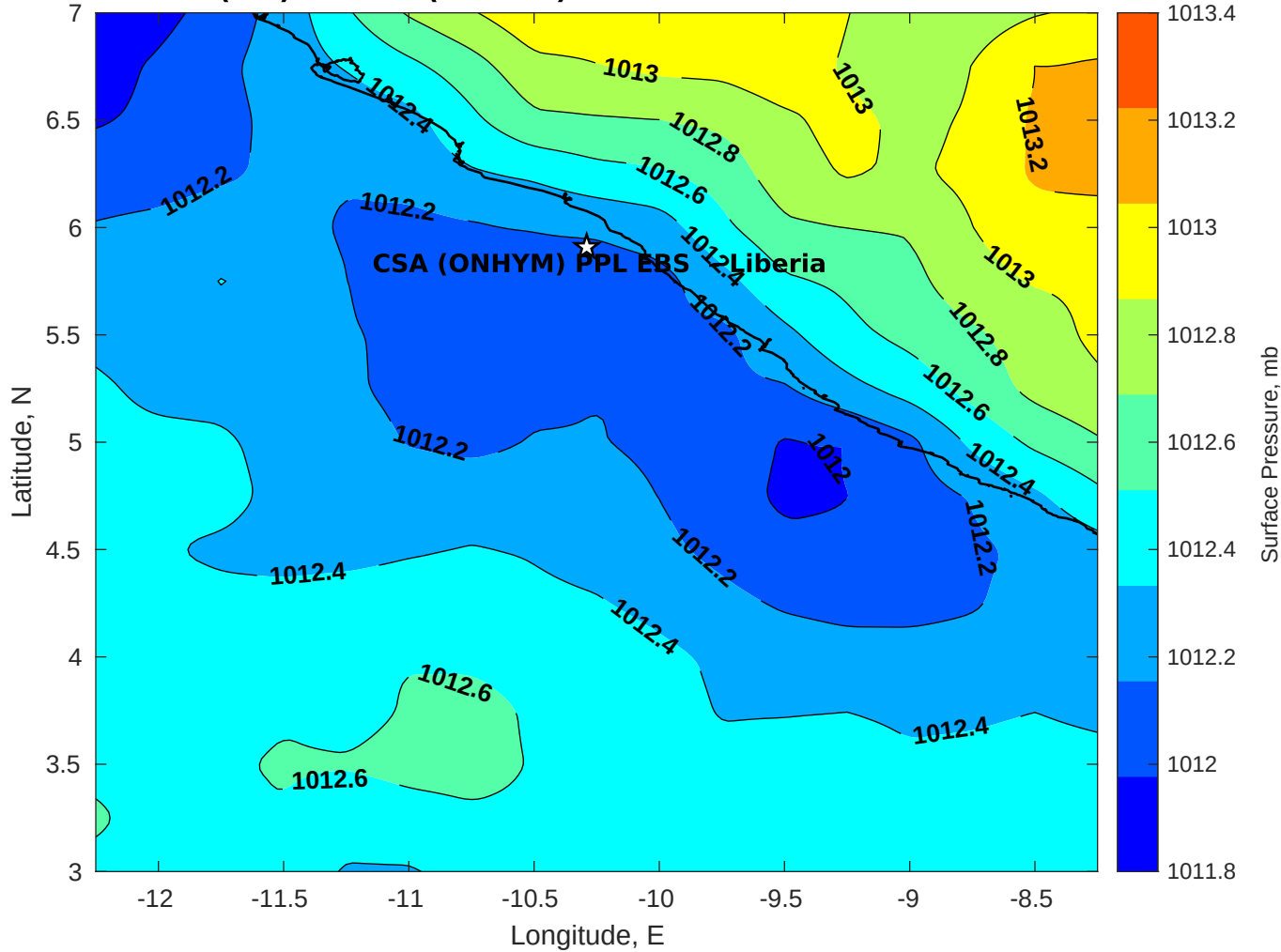
Surface Pressure (mb) for CSA (ONHYM) PPL EBS - Liberia at 23-Nov-2025 00:00:00
