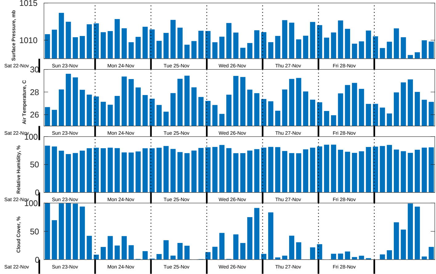
Met Forecast for CSA (ONHYM) PPL EBS - Liberia from 23-Nov-2025 00:00:00 to 30-Nov-2025 00:00:00
