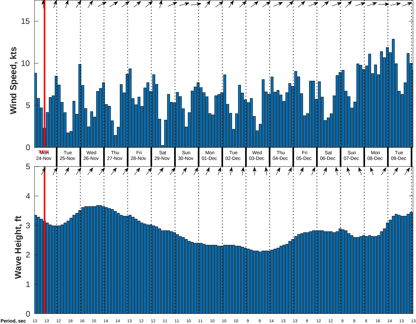
Wind & Wave Forecast for CSA (ONHYM) PPL EBS - Liberia from 23-Nov-2025 01:00:00 to 09-Dec-2025 01:00:00
