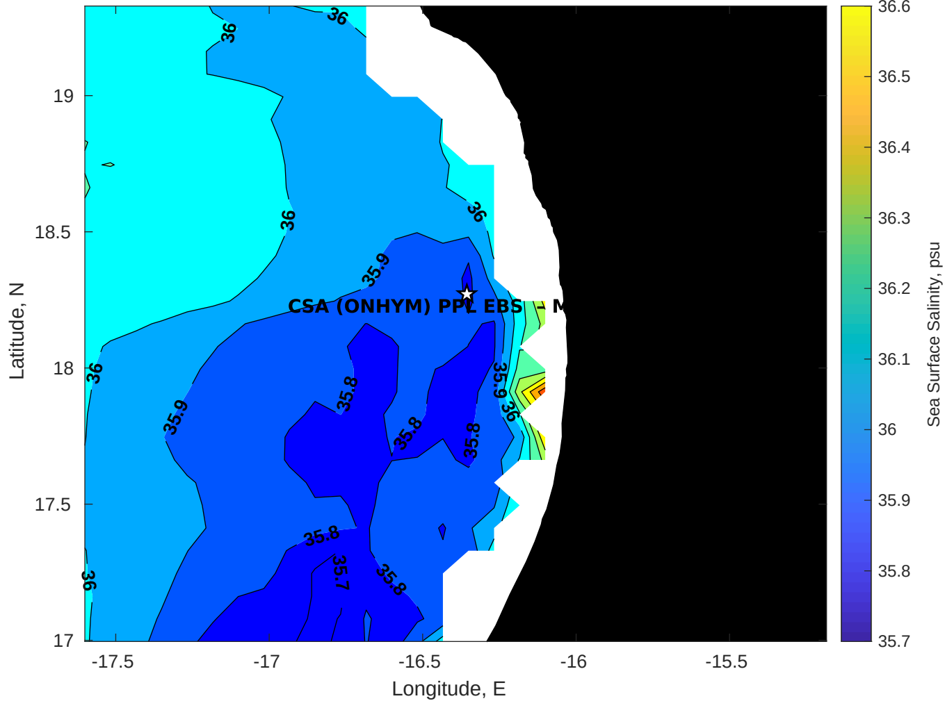
Surface Salinity for CSA (ONHYM) PPL EBS - Mauritania at 22-Nov-2025 00:00:00
