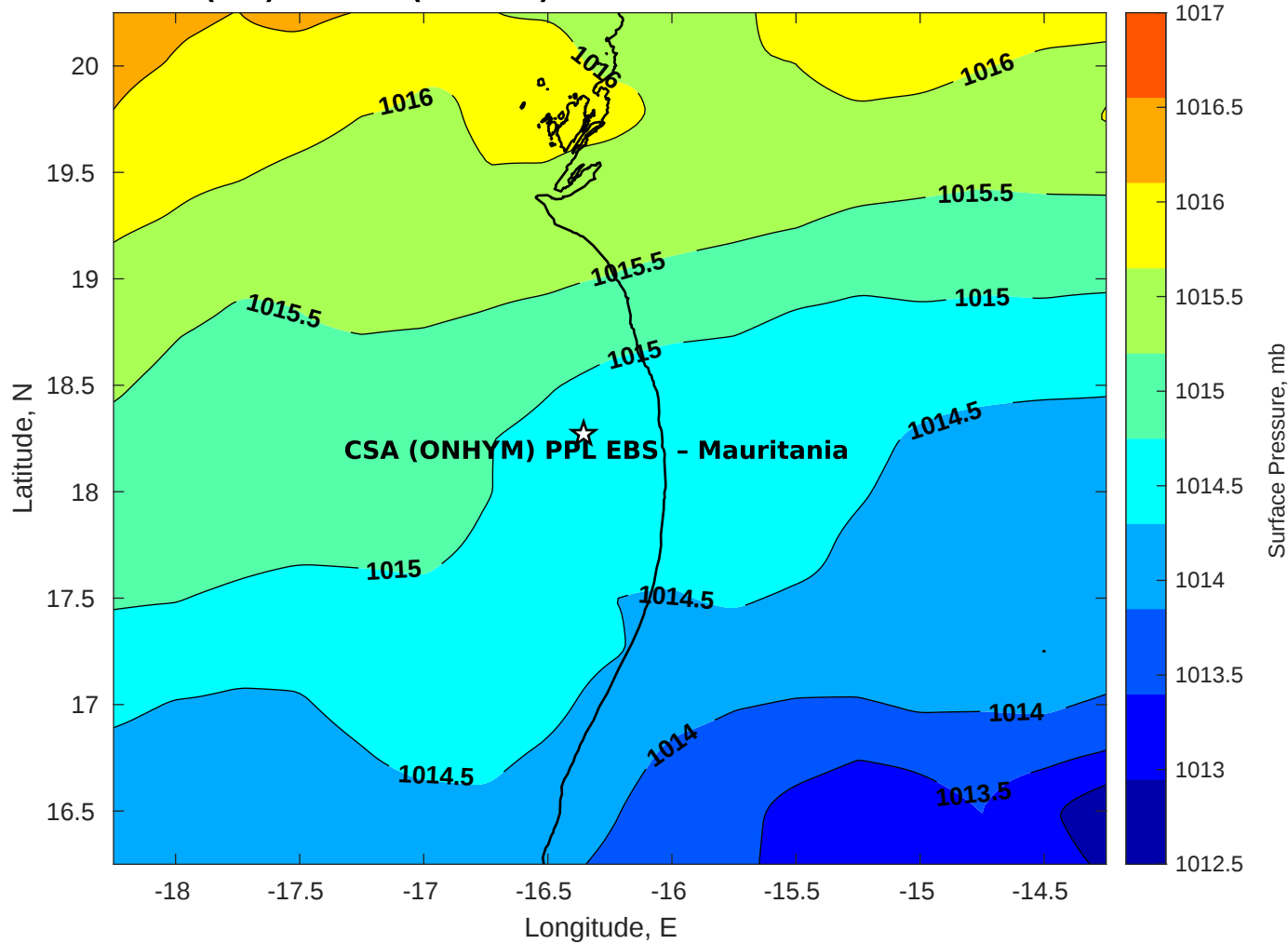
Surface Pressure (mb) for CSA (ONHYM) PPL EBS - Mauritania at 23-Nov-2025 00:00:00
