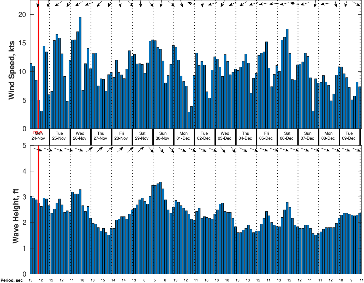
Wind & Wave Forecast for CSA (ONHYM) PPL EBS - Mauritania from 23-Nov-2025 01:00:00 to 09-Dec-2025 01:00:00
