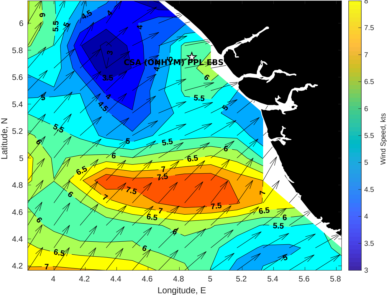
GFS Winds (kts) for CSA (ONHYM) PPL EBS - Nigeria at 23-Nov-2025 09:00:00
