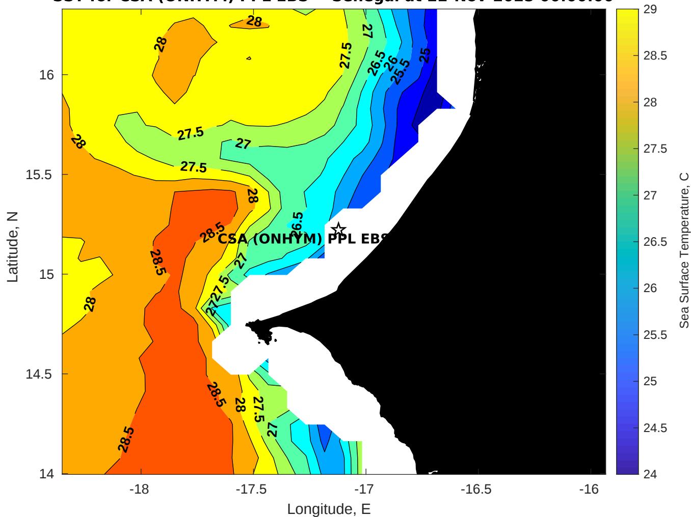
SST for CSA (ONHYM) PPL EBS - Senegal at 22-Nov-2025 00:00:00
