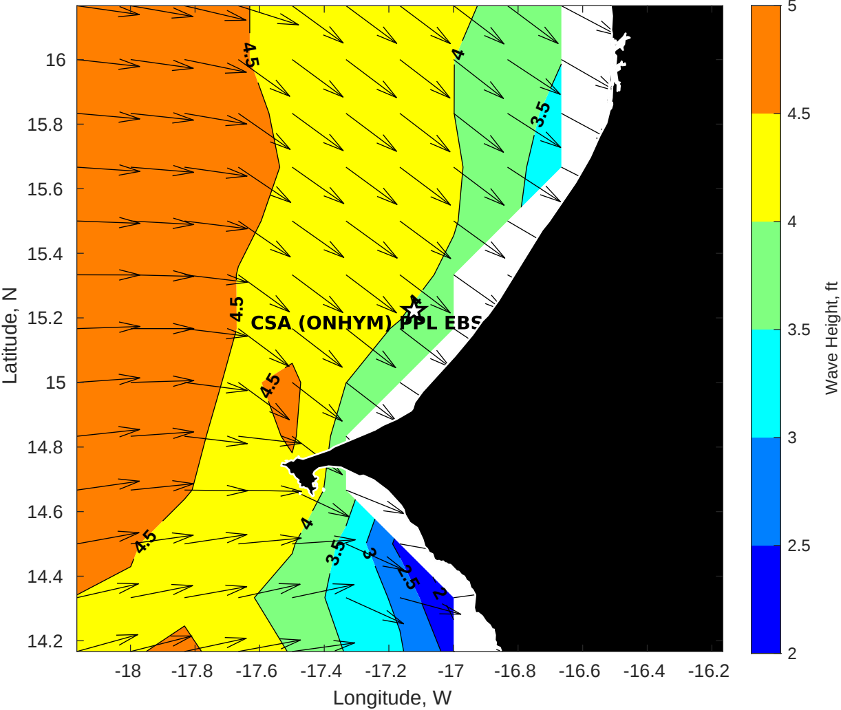
GFS Wave Height (ft) for CSA (ONHYM) PPL EBS - Senegal at 23-Nov-2025 09:00:00
