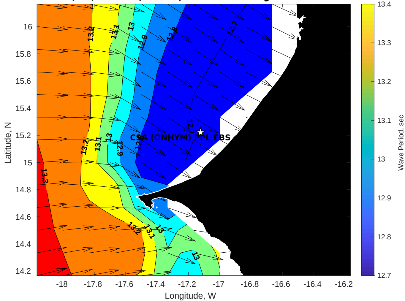
GFS Wave Period (sec) for CSA (ONHYM) PPL EBS - Senegal at 23-Nov-2025 09:00:00
