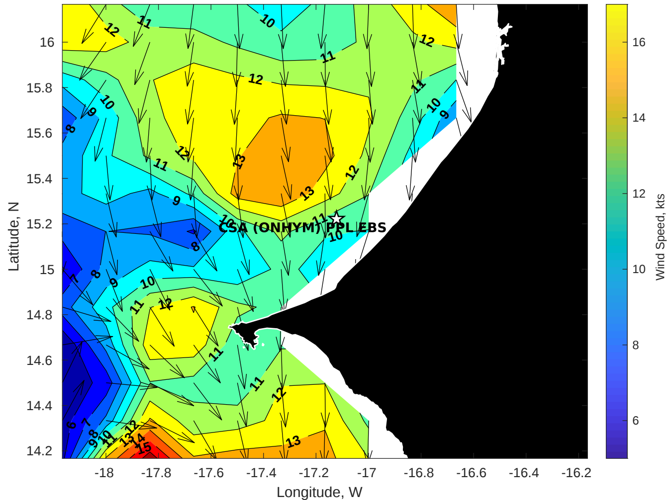
GFS Winds (kts) for CSA (ONHYM) PPL EBS - Senegal at 23-Nov-2025 09:00:00
